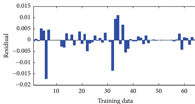
FIGURE 6: Residuals between ANN and experimental data for training data.
