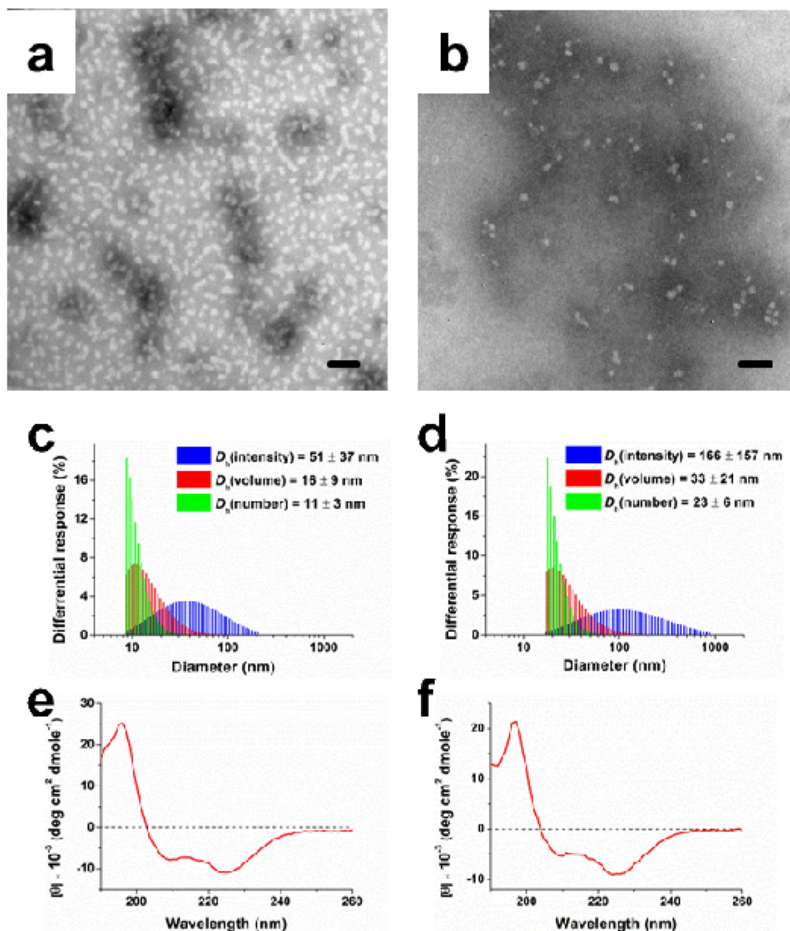
Fig. 2. TEM images for cationic 6 (a) and anionic 7 (b) nanoparticles. The scale bars in both TEM images are 50 nm. (c) DLS results of cationic nanoparticles 6 : D_h (intensity) = 51 \pm 37 nm, D_h (volume) = 16 \pm 9 nm and D_h (number) = 11 \pm 3 nm. (d) DLS results of anionic nanoparticles 7 : D_h (intensity) = 166 \pm 157 nm, D_h (volume) = 33 \pm 21 nm and D_h (number) = 23 \pm 6 nm. CD spectra of 4 (e) and 5 (f) in nanopure water at a polymer concentration of 0.1 mg/mL.
