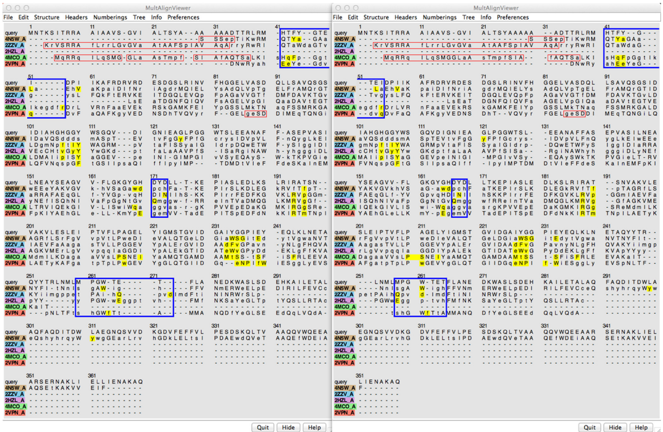
Figure 2. Side-by-side comparison of the BLAST pseudo-MSA (left) and the MSA from Clustal Omega (right) of the query and chains A of 4N5W, 2ZZZ, 2HZL, 4MCO and 2VPN. Each alignment is displayed in a Multalign Viewer window in Chimera. Residues within 5 Å of the respective bound ligands are highlighted in yellow. Residues missing from the 3D structures are enclosed in red outline boxes. Clustal Omega was run using one iteration and full distance matrices during the initial alignment and iteration. Blue rectangles outline some of the places where binding-site residues in the template structures (yellow) are aligned differently with the query sequence, which would give rise to different binding-site residues in the resulting comparative models.
