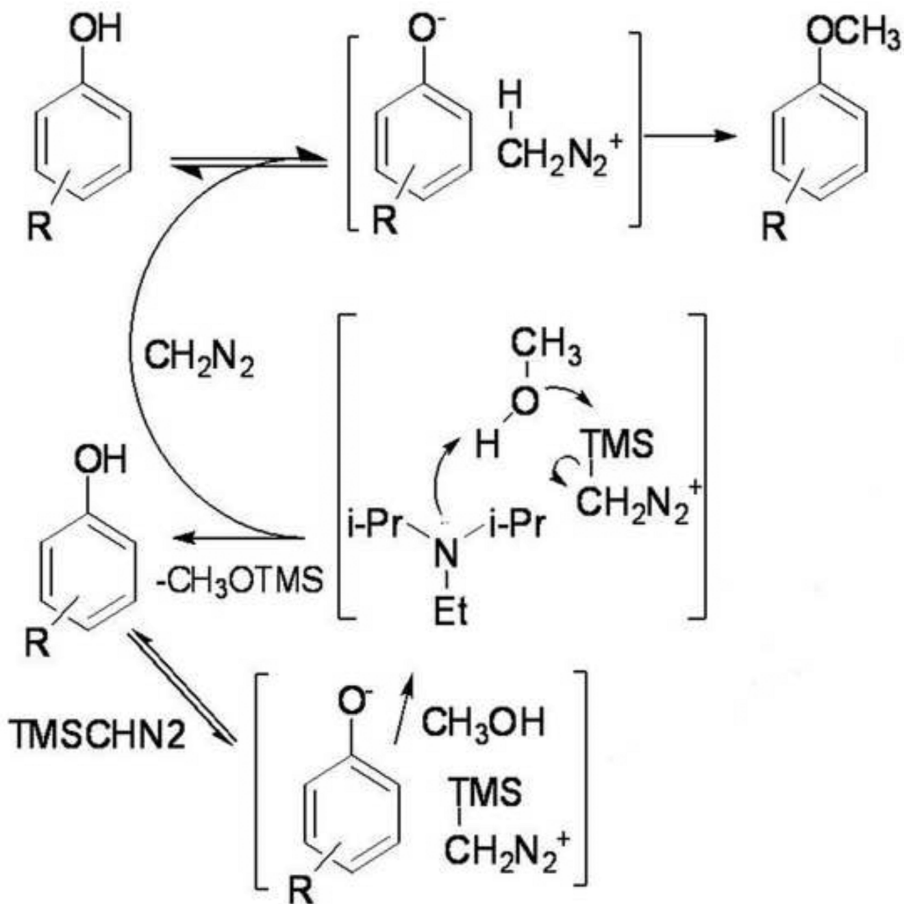
Figure 6. Proposed reaction mechanism of the O-methylation with TMS-DM and DM as based on Kuehnel et al , 2007. The mechanism shows the abstraction of a hydrogen from the phenol with subsequent in situ generation of diazomethane which after a second hydrogen abstraction can react with the hydroxyl group of the analyte to form a methoxy derivative.
