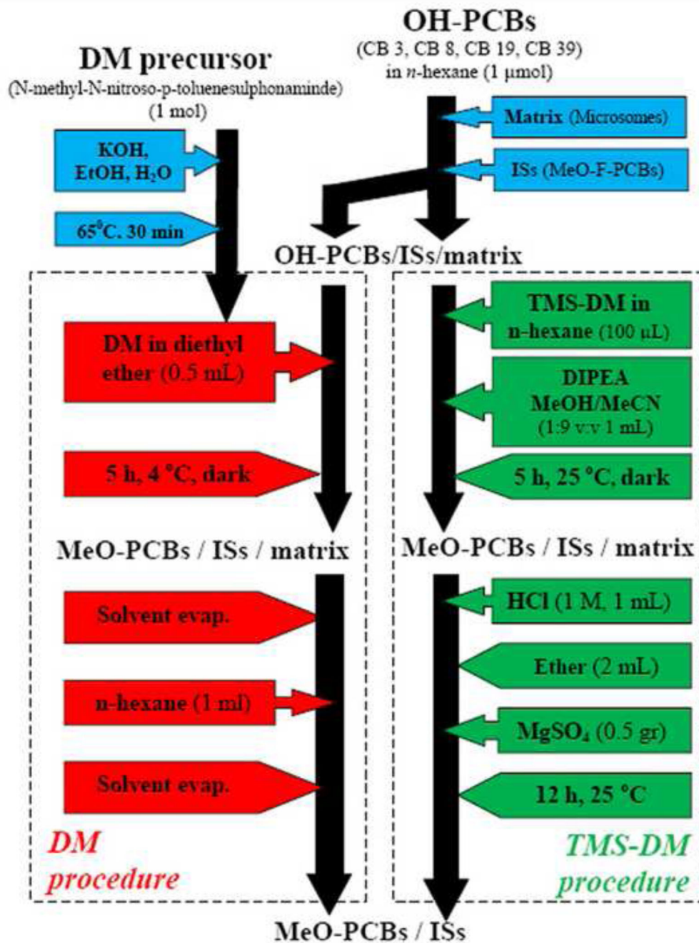
Figure 2. General workflow chart showing the DM and TMS-DM derivatization procedures.
