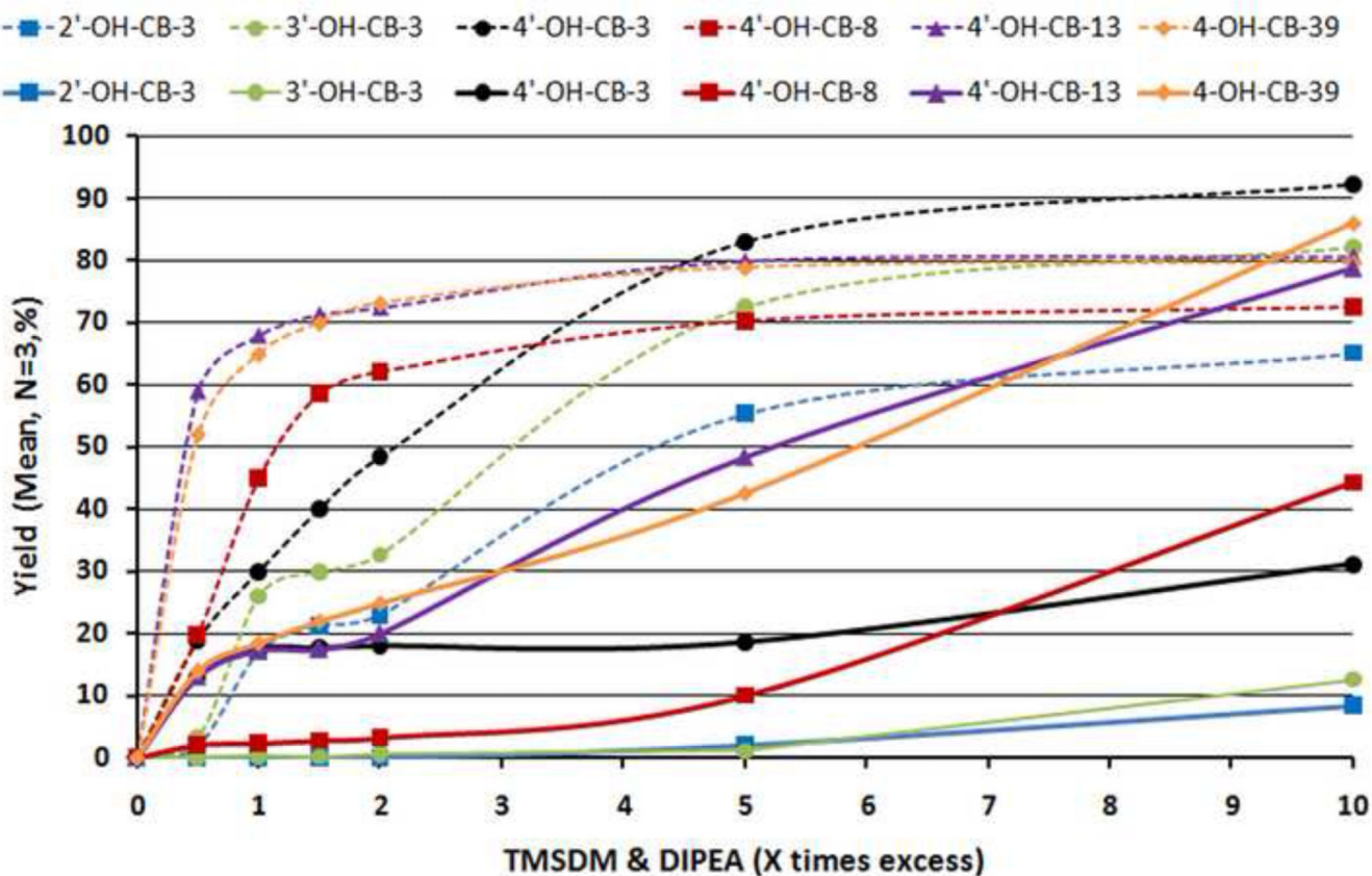
Figure 3. Yields of the derivatization of OH-PCBs (2'-OH-CB-3, 3'-OH-CB-3, 4'-OH-CB-3, 4'-OH-CB-13, 4'-OH-CB-8, 4-OH-CB-39) by TMS-DM at various conc. of TMS-DM and DIPEA in a real matrix (MeCN/MeOH (9:1) + denatured microsomal fraction extract) ( solid line ) compared to a reference matrix (MeCN/MeOH (9:1)) ( dotted line ) determined by GC-MS, utilizing MeO-F-PCBs analogues (4'-MeO-CB-3-F3, 3'-MeO-CB-3-F3, 2'-MeO-CB-3-F3, 4'-MeO-CB-13-F3, 4'-MeO-CB-8-F3, 4-MeO-CB-39-F3') as internal standards. The reaction time was a constant 24 h. Standard deviation range was between 0.002 and 0.2 %.
