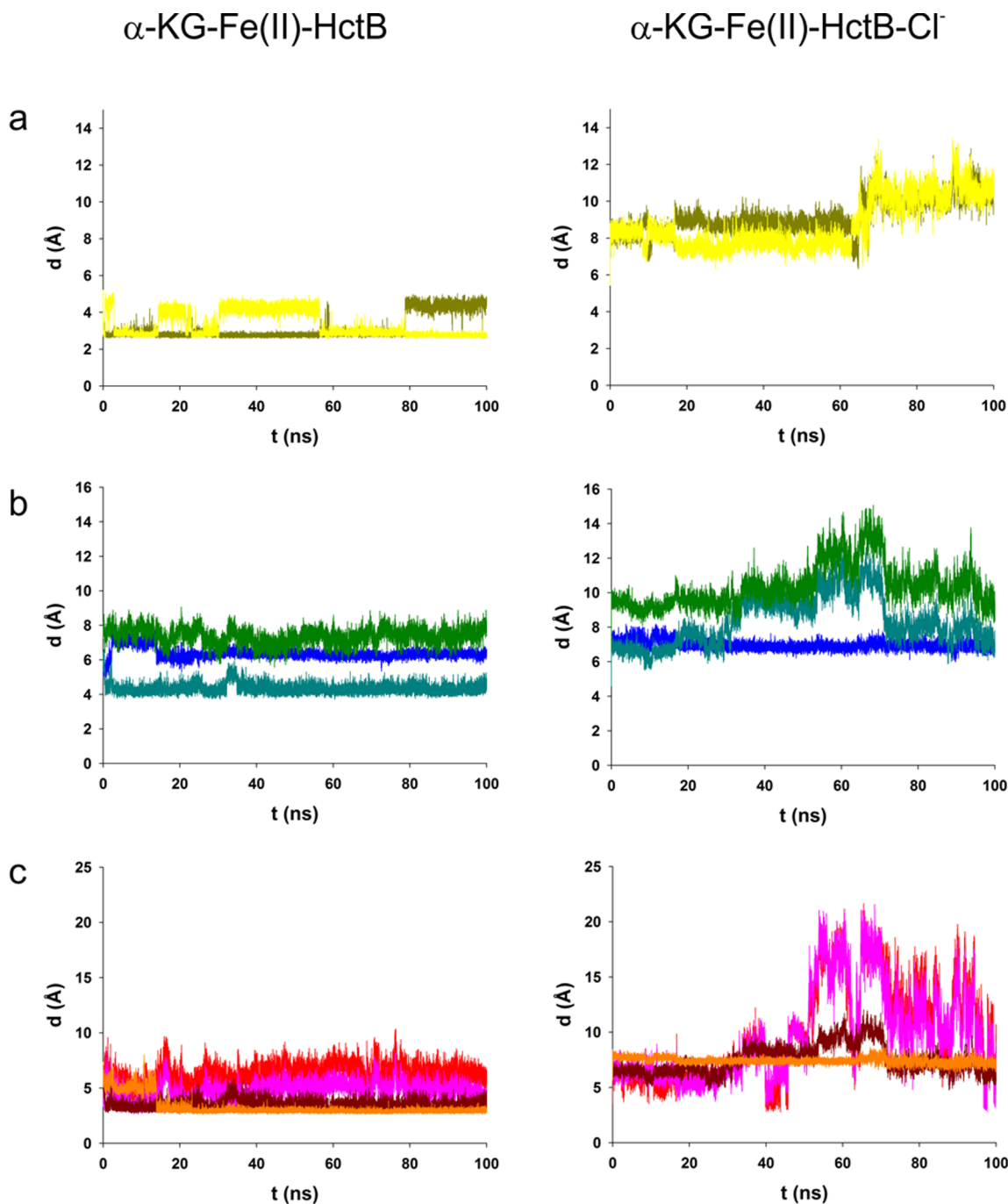
Figure 8. Trajectories from 100 ns MD simulations depicting distances of residues involved in the chloride-triggered structural rearrangement in HctB in the absence (left panels) and presence (right panels) of 1 M chloride. Panel a shows distances of O-5 and O-5' of Glu224 to Fe(II). Panel b displays backbone distances from C-2 of Asn140 to N-2 of Glu224 (blue); N-2 of Val114 to C-2 of Glu224 (teal); and C-2 of Tyr115 to C-2 of Arg225 (green). Panel c gives the distances of the putative H-bonding atoms O-7 of Tyr115 to N- \omega of Arg225 (red); O-7 of Tyr115 to N- \omega' of Arg225 (pink); N-2 of Val114 to O-1 of Glu224 (dark red); and O-4 of Asn140 to N-2 of Glu224 (orange).
