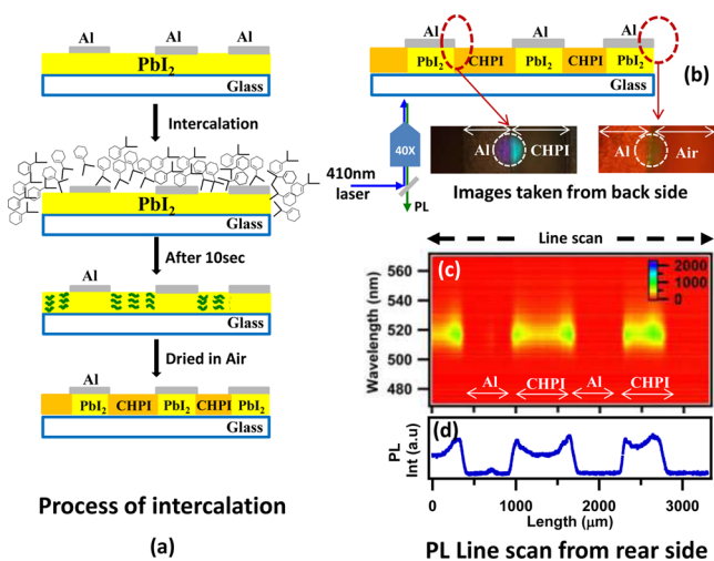
Figure 5. (a) Scheme of intercalation into \text{PbI}_2 film coated with Al metal strips. (b) PL line mapping performed from the backside of the glass substrate and the corresponding confocal PL images obtained using a 410 nm diode laser. (c, d) Corresponding PL image plot and PL peak intensity across the structures.
