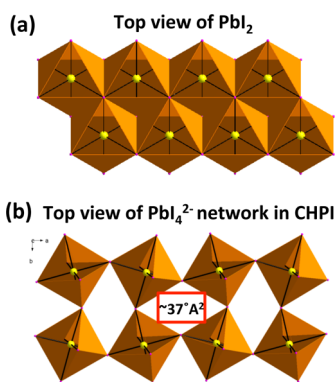
Figure 6. Schematic representation of crystal packing in (a) \text{PbI}_2 and (b) inorganic layers of CHPI ( \text{PbI}_4^{2-} network) seen along the c -axis. ( \text{PbI}_2 space group is P\bar{3}m1 with a = 4.555 \text{ \AA} , b = 4.555 \text{ \AA} , and c = 6.977 \text{ \AA} and CHPI space group is P\bar{1} , a = 12.2053 \text{ \AA} , b = 12.3053 \text{ \AA} , and c = 18.3182 \text{ \AA} ). 43,44
