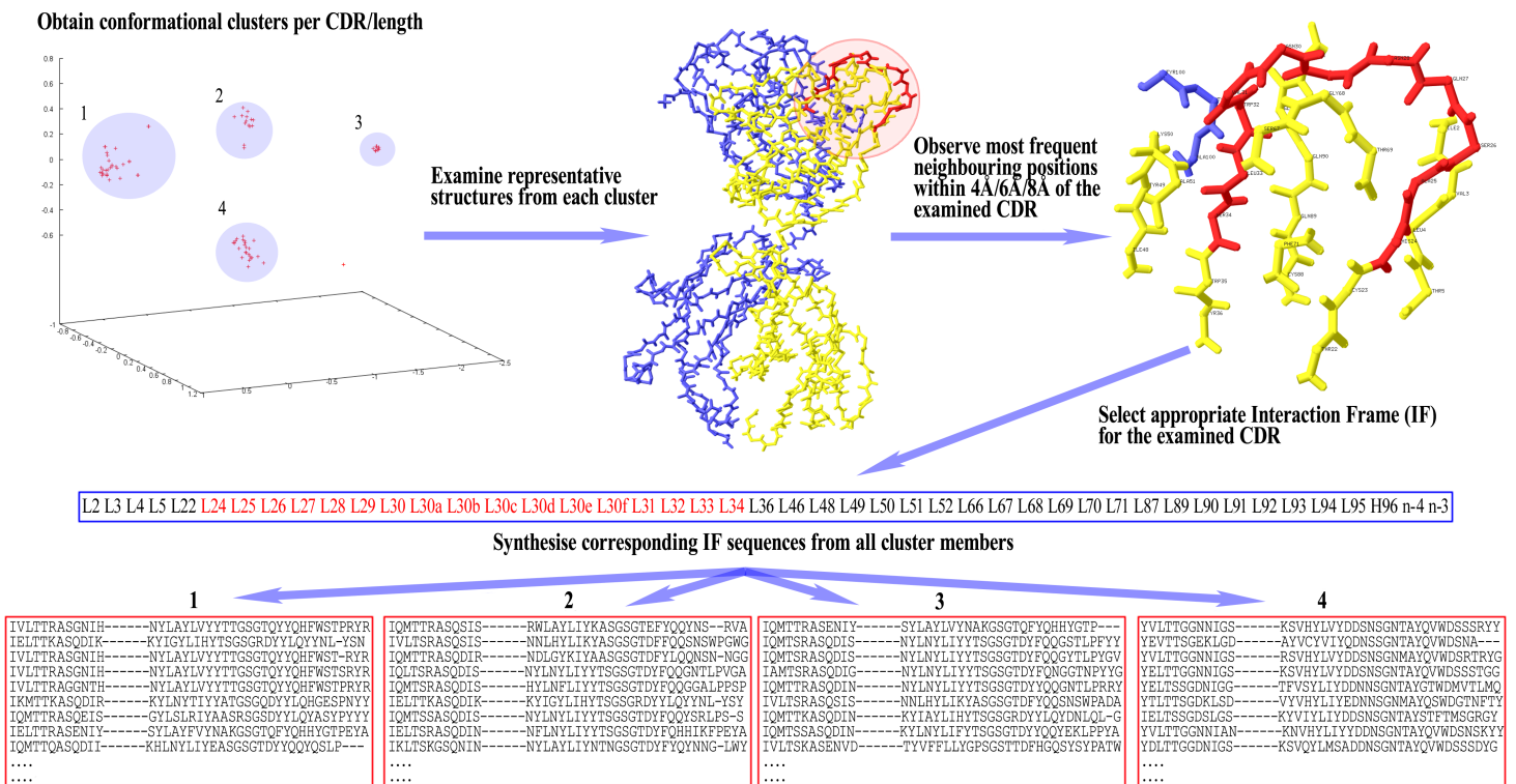
Figure 1 Preparatory steps for DCP. Here, an Interaction Frame (IF) is selected for CDR-L1 and the corresponding IF sequences are synthesised for each one of the four clusters of the given length. For computational reasons the same IF is defined for all lengths of any given CDR (here, CDR-L1 for illustration purposes). Therefore, observed gaps in IF sequences correspond to insertions populated in longer lengths than the one shown in the illustrated example—gaps are filled accordingly in those lengths' IF sequences. Spare gaps, on the other hand, may correspond to IF positions pointing to unpopulated insertions from other CDRs or deletions in the Fv sequence. Also, gaps are present if there is no Light or Heavy chain in that particular structure. Positions at the end of the IF, marked as 'n - x', refer to CDR-H3 positions at a sequential distance x from the last residue n (H102; see text).
