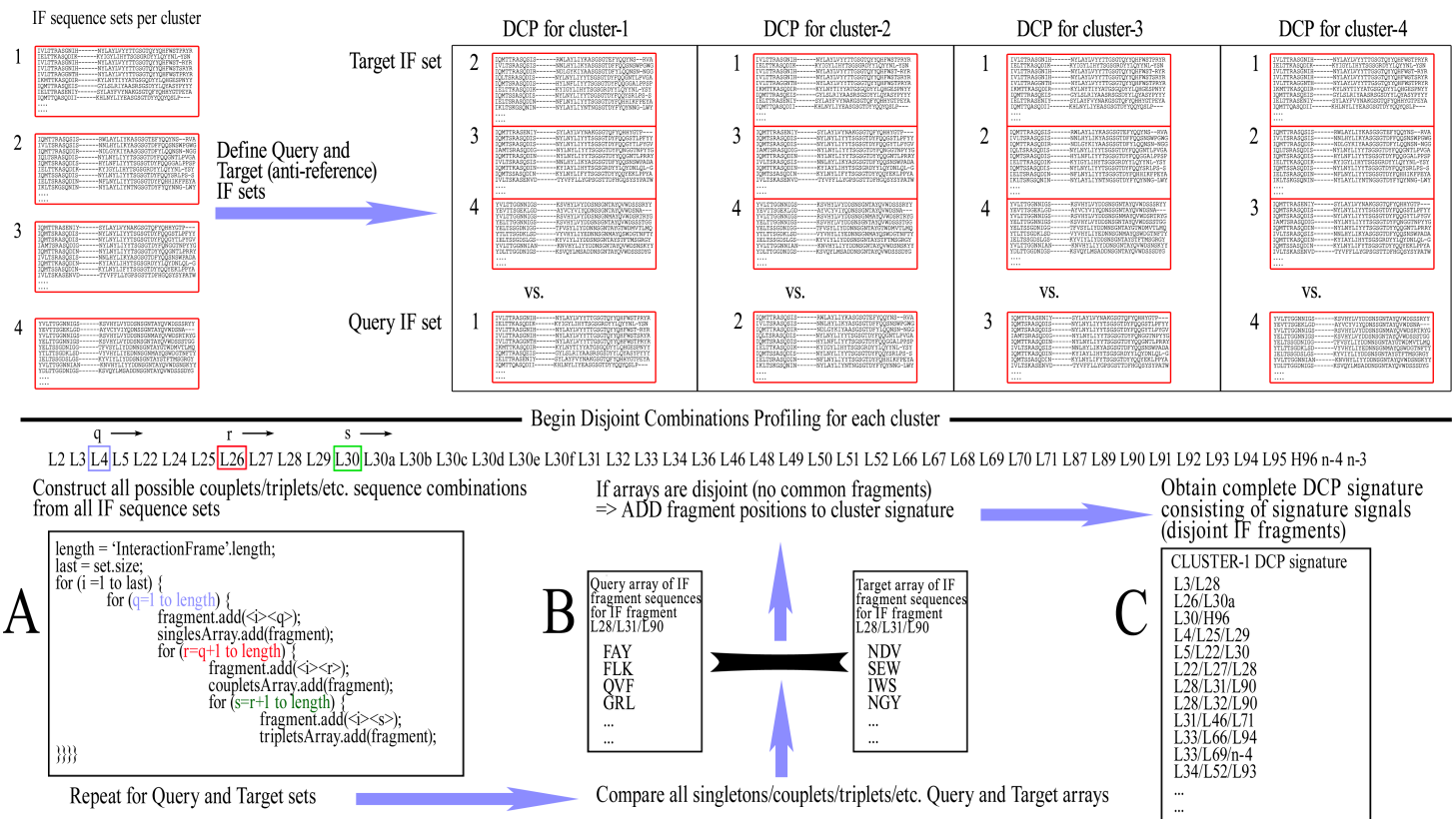
Figure 2 The training procedure using Disjoint Combinations Profiling. Definition of Query and Target IF sequence sets, extraction of all available IF fragment sequences and comparison between corresponding sets of fragments for disjointness, leading to signature signals.
