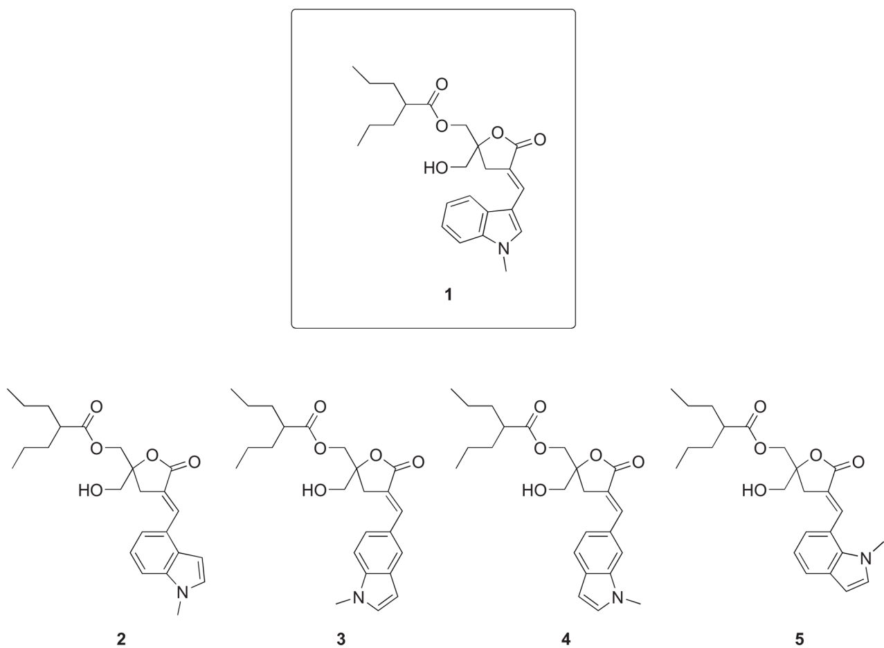
Figure 1. Structures of DAG-indololactones.
