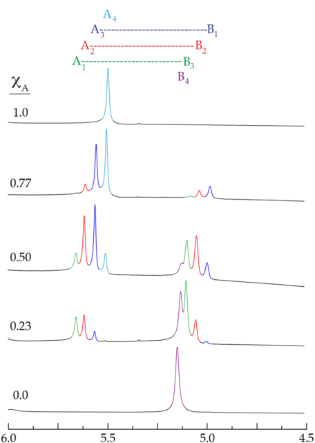
Figure 6. ^1\text{H} NMR spectra of sodium enolates 11 (A) and 13 (B) at 0.10 M total concentration in 0.50 M TMEDA/toluene- d_8 at varying X_A recorded at -80 °C.
