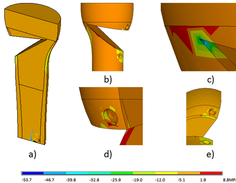
Figure 3 The distribution of stresses in the \sigma_z plane in the bone in the entire volume (a) and in the zones of stress concentration (b-e) for the osteosynthesis with the first generation Puddu plate.
