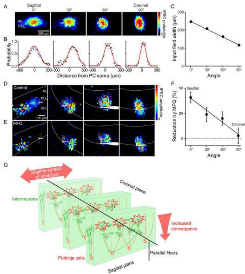
Figure 7. Electrical coupling between interneurons is spatially biased
