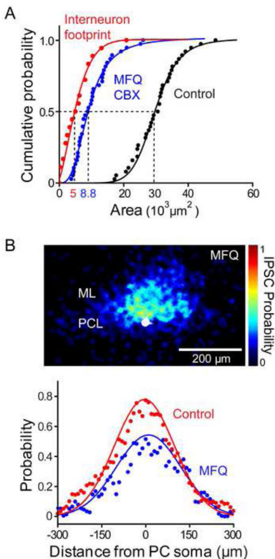
Figure 6. Quantification of the contribution of electrical synapses to interneuron convergence (A) Calculation of amount of convergence of interneuron inputs onto a PC, as in Figure 3G, in control conditions (black) or in the presence of a gap junction blocker (CBX or MFQ; blue, n = 38 ). Median area of input fields measured after blocking electrical synapses ( 8.8 \times 10^3 \mu\text{m}^2 ) was almost 3-fold smaller than in control conditions ( 3.0 \times 10^4 \mu\text{m}^2 ), but was 1.8-fold larger than the area of MLI optical footprints ( 5.0 \times 10^3 \mu\text{m}^2 , n = 18 ) measured in the presence of gap junction blockers (red). This indicates that MLI circuits providing inhibitory inputs to a PC consist of roughly 2 direct chemical synapses with several additional MLI converging via electrical synapses.
