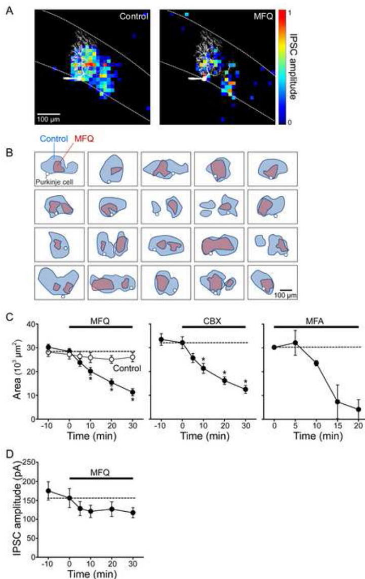
Figure 4. Electrical synapses contribute to inhibitory input field of Purkinje cells (A) The area of the inhibitory input field of a PC (left panel) was reduced by treatment with MFQ (50 \mu M; right panel). Pseudocolor scale indicates the normalized amplitude of light-evoked IPSCs for each location. Image of dye-filled PC is shown in white. (B) Gallery of input field maps measured for 20 different PCs before and after MFQ treatment. Outlines of input fields measured in control conditions are shown in blue and those measured in the same experiments after MFQ treatment are shown in pink. In every case, MFQ treatment reduced the area of the input field. White circles indicate the location of somata of PCs used for input field determinations. (C) Time course of changes in the mean area of inhibitory input field of IPSCs during MFQ (50 \mu M, n = 20), CBX (200 \mu M, n = 18) and MFA (200 \mu M, n = 2) treatment. Asterisks indicate time points where drug treatment caused significant ( p < 0.001 ) reductions. (D) Time course of changes in the mean IPSC amplitude during MFQ treatment (50 \mu M, n = 20).
