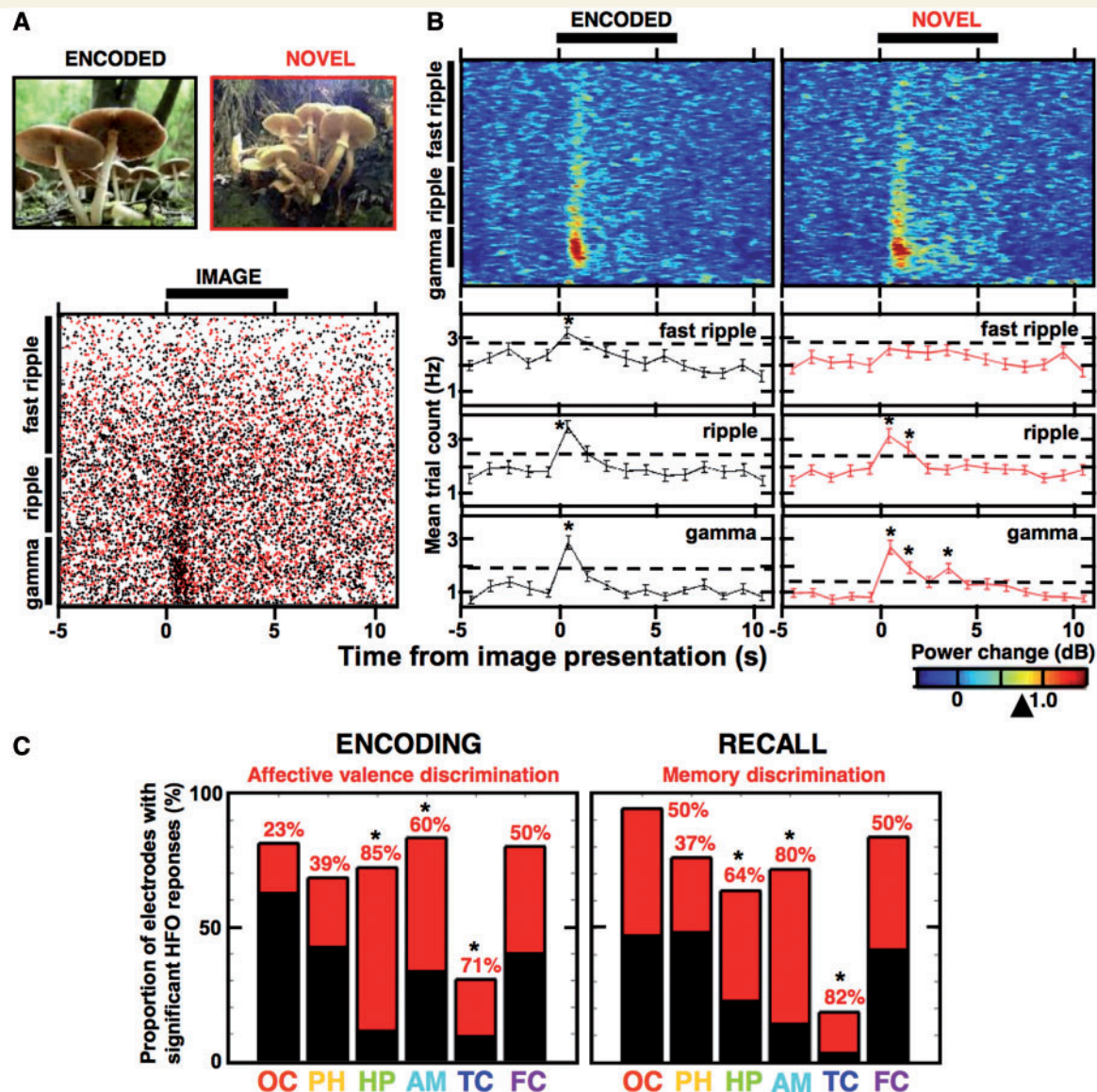
Figure 7 Induced HFOs reveal discriminative responses to the encoded images. ( A , top) Examples of two similar pictures (analogous to the International Affective Picture System (IAPS) set of images used in the study, which were not allowed for publication)—one previously seen during encoding (black code) and the other novel (red code); ( A , bottom) cumulative scatterplot of all HFO detections in the three frequency bands recorded from an example amygdala electrode in Patient 8 during his memory recall—black dots were detected from trials with encoded images and the red dots from trials with novel images of the same session (black bar indicates the time-course of image presentation). ( B , top) Spectrograms summarize trial-averaged power changes (plotted as in Fig. 2) in the two trial types from the scatterplot in A , ( B , bottom) the mean trial counts for the scatterplot in A (see Fig. 2) are summarized separately for the gamma, ripple and fast ripple detections, aligned to the trial time-course of the spectrograms. Notice significant induction of the HFOs in individual bins as compared to matched average count from the five 'baseline' bins (Wilcoxon signed-rank test, *P < 0.01 , encoded: 77 trials; novel: 55 trials), which is not present in the fast ripple response to novel images and was significantly different from the fast ripple response to encoded images (Friedman ANOVA, eight time bins, 55 trials, P = 0.013 ; see Fig. 2). ( C ) Proportion of all electrodes that showed discriminative HFO responses (as in B ) to affectively charged images during encoding (left) and to the encoded images during recall (right) are summarized across the studied structures (the total black bar indicates number of electrodes with significantly induced HFOs and its red part indicates fraction of these electrodes that showed significant differences; see Supplementary Table 1). Notice that the highest fraction of electrodes with the discriminative HFO responses is reported in the hippocampus, amygdala and the temporal cortex, consistently exceeding 50% (marked with asterisk).
