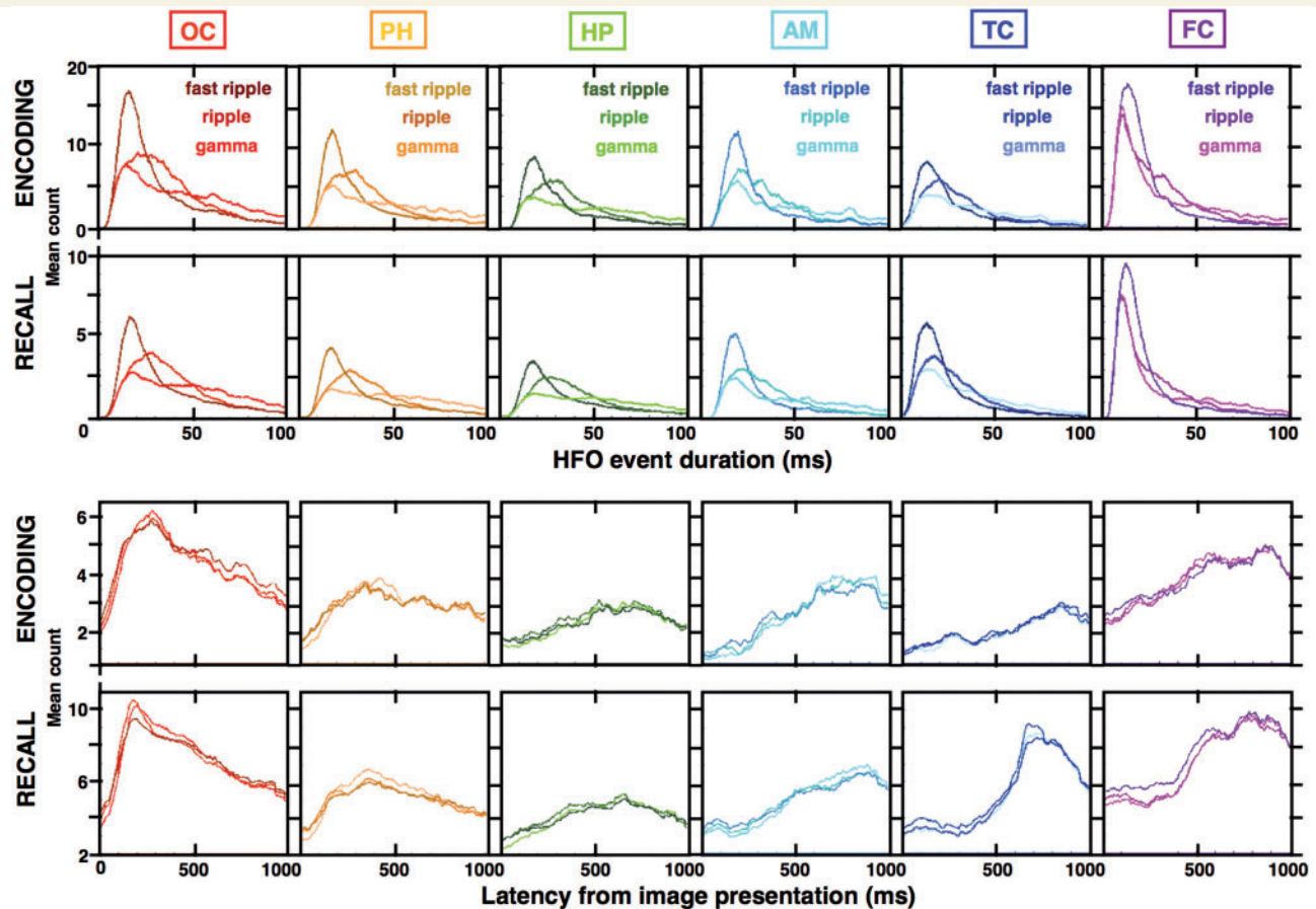
Figure 5 The high gamma, ripple and fast ripple induced HFOs have distinct durations and consistent latencies from image presentation. Distributions of all induced HFO detections from Fig. 4 (from the encoding stage of the task) were broken down into the high gamma, ripple and fast ripple bands and presented together with all the detections from the recall stage [ n = 18\,095 occipital (OC), 13\,755 parahippocampal (PH), 9\,317 hippocampal (HP), 4\,965 amygdala (AM), 7\,706 temporal cortex (TC), 6\,729 frontal cortex (FC) detections]. (A) Histogram counts of gamma, ripple and fast ripple HFO durations reveal distinct population distributions with significantly different means in every color-coded structure (gamma > ripple > fast ripple, Wilcoxon rank sum test, P < 0.01 ). The average HFO duration in each band corresponds to \sim 4 – 10 cycles of oscillation. (B) The three HFO bands show overlapping distributions of the mean latency trial counts from image presentation and show the same progression along the visual processing stream as in Fig. 4—the sharp induction of the occipital HFOs early after image presentation, followed by gradual accumulation in subsequent structures of the visual stream with late peaks in the temporal and frontal cortices. Plots in the figure were smoothed using a moving sliding average of 10 samples to facilitate data interpretation. Notice that the durations and latencies were consistent in the encoding and recall stage of the task in all structures except for temporal and frontal cortex, where HFO latencies were significantly longer during memory recall (see Fig. 6 for memory modulation of the HFO counts in the six structures during the two task stages).
