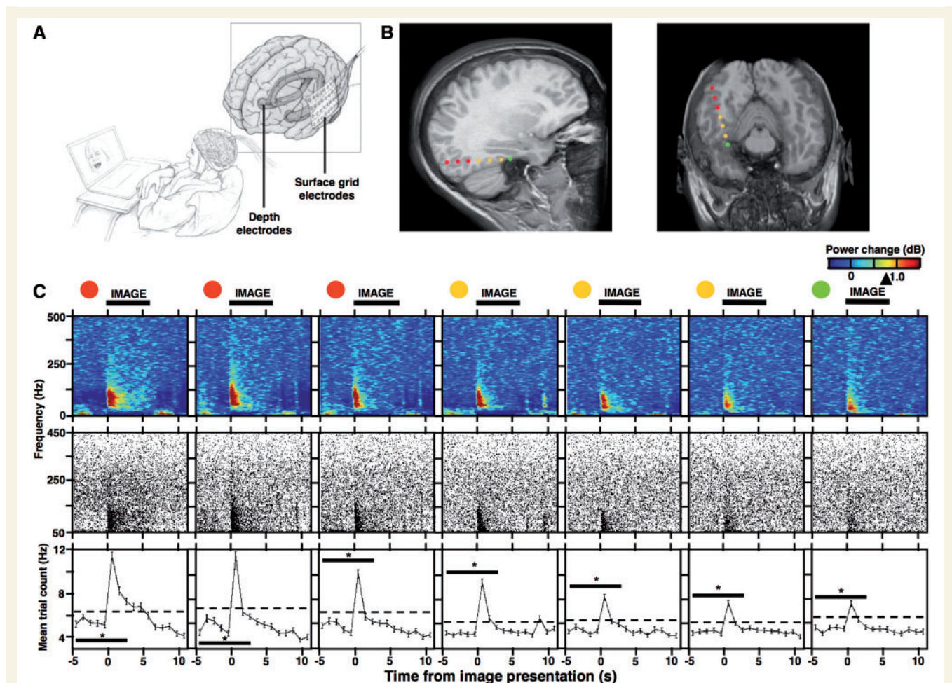
Figure 2 Quantification of cognitively induced HFOs. (A) Sketch of the experimental setup for intracranial patient recordings during the visual recognition memory task. (B) MRI scans show localization of seven bipolar depth-electrode recording sites (reconstructed from a high resolution CT images of the original eight contact points; see Burke et al. , 2013) in the right occipital cortex (red), parahippocampal cortex (orange), and the hippocampus (green) from Patient 10. (C, top ) Spectrograms of normalized trial-averaged power changes ( n = 140 trials; obtained with the multi-taper spectral analysis) were obtained from the seven bipolar recording sites in B (colour-coded) during memory encoding (image presentation time indicated by the horizontal black bar; arrowhead on the power scale points to Jack-knifed upper error estimate at P < 0.01 significance level); (C, middle ) cumulative scatterplots show HFO detections from individual trials (140 trials; detected with the Hilbert spectral analysis method—each black dot is one detection – see Fig. 3 and ‘Materials and methods’ section for more details) aligned to the time axis of the spectrograms (notice the close overlap between the activation pattern in trial-averaged power spectrograms and the cumulative HFO scatterplots obtained with the multi-taper and Hilbert transform spectral analyses, respectively); (C, bottom ) the HFO detections from the middle panel were summarized as mean trial counts and binned across the same time-axis (dashed line indicates 3 SD above the mean of the five ‘baseline’ bins preceding the image onset). The mean counts from these five baseline bins and the following three bins that overlapped with image presentation (indicated by black significance bar) were used to quantify significant induction of HFO detections (Kruskal-Wallis test, eight time bins, 140 trials, *P < 0.01 ). Notice that in this example all of the electrodes from the three structures showed significant inductions of HFO discharges, overlapping with the profile of significant induction in the trial-averaged power spectrograms (see Supplementary Fig. 2 for another example of prefrontal cortical electrode response).
