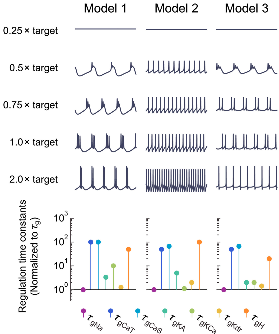
Figure 5. Changing Targets within Cell Types
