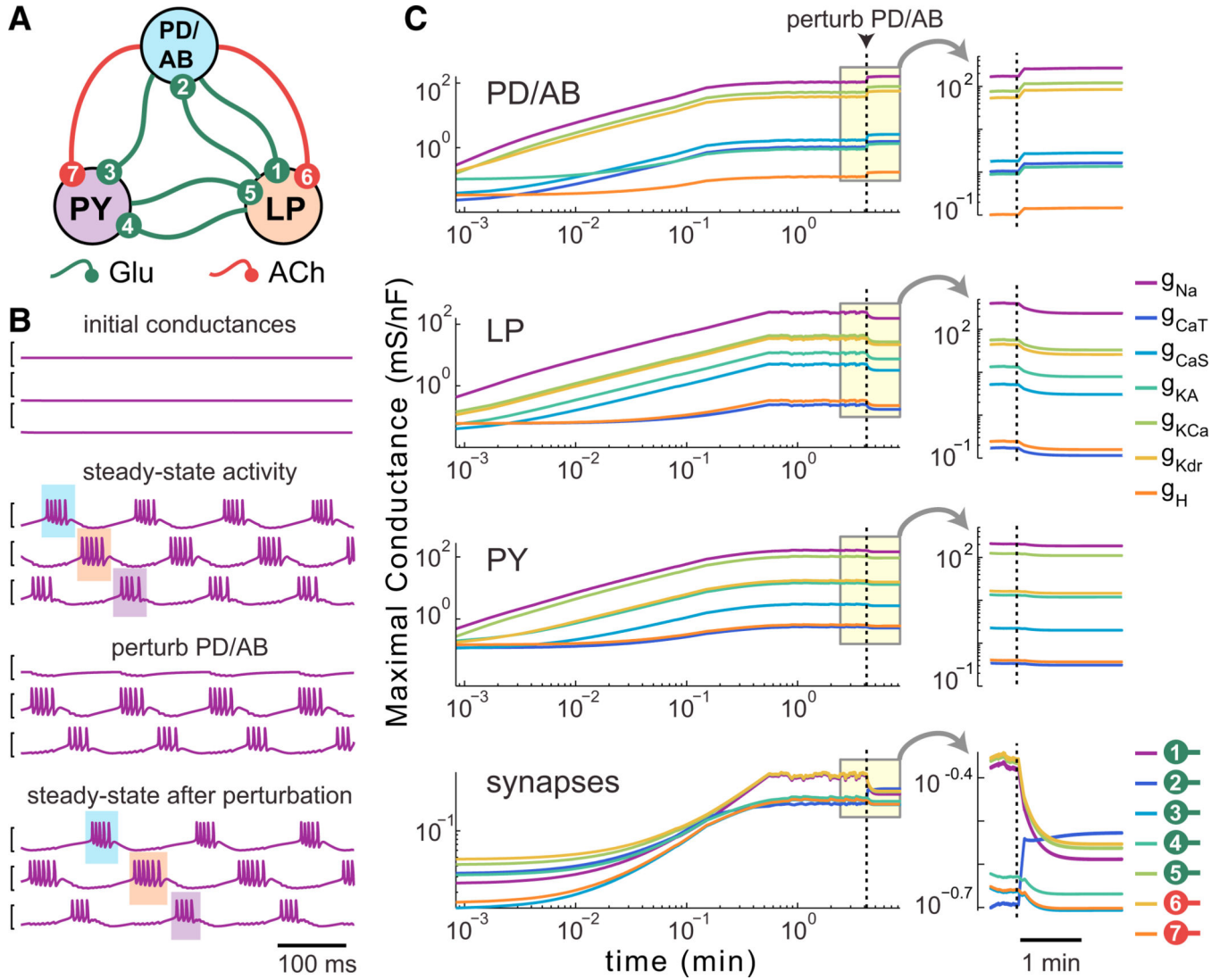
Figure 6. A Self-Assembling, Self-Regulating Central Pattern Generating Network
