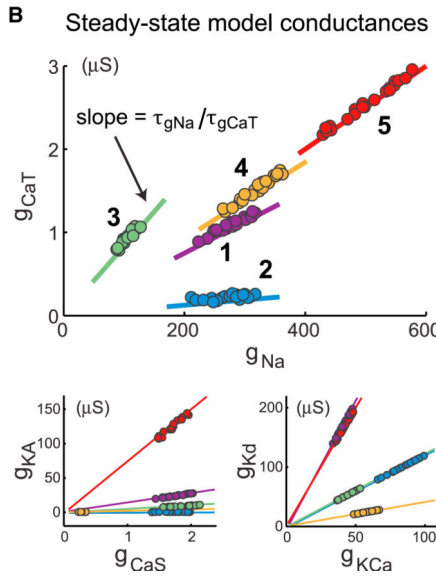
Figure 4. Specifying Different Cell Types with the Same Model
