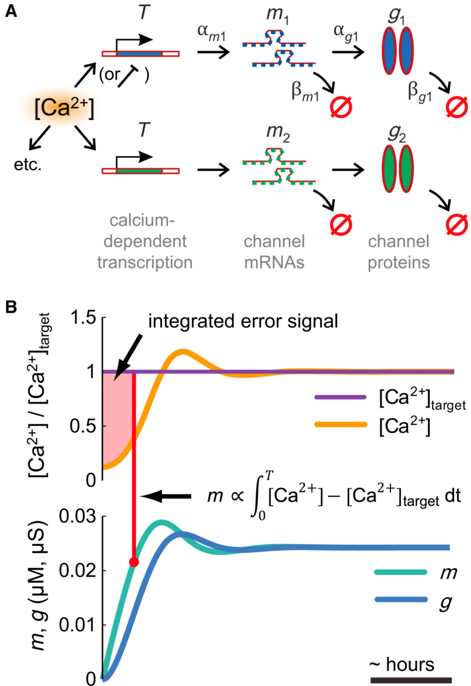
Figure 1. Integral Control from the Canonical Model of Gene Expression
