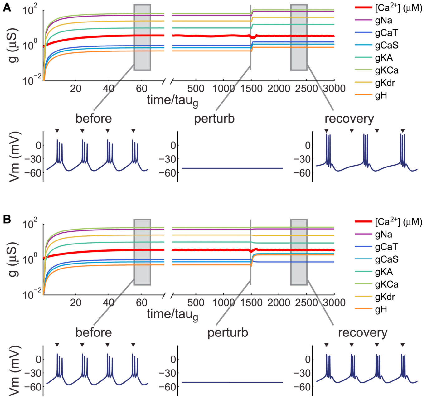
Figure 8. Switching Regulation Rates in the Same Cell Can Preserve Specific Properties (A) Conductance regulation in a bursting pacemaker neuron. Membrane potential traces (500 ms duration) are shown at steady state, at the onset of a perturbation (hyperpolarizing leak), and at steady state following perturbation. Arrowheads above the rightmost trace indicate burst onset times of the unperturbed neuron, aligned to the first burst. (B) Evolution of the same model as (A), but with regulation rule switched prior to the onset of the perturbation. Regulation time constants following the switch were chosen to preserve burst duration (see Experimental Procedures). Arrowheads as in (A). Membrane potential trace durations: 500 ms.
