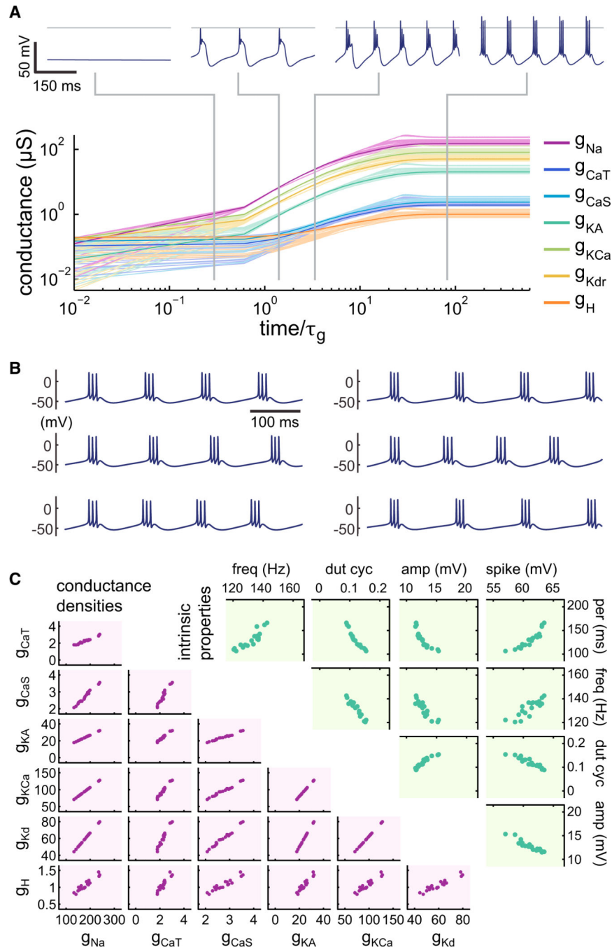
Figure 3. Regulation in a Complex Biophysical Cell Model
