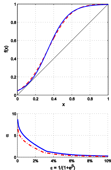
Fig. 7. (Upper) Logit response function (blue solid line) and normally distributed payoff shocks (red dashed line) ( \alpha = 1 , \epsilon = 5\% ). (Lower) Thresholds for topology-free fast diffusion: logit (blue solid line) and normally distributed payoff shocks (red dashed line) ( d = 15 ).
