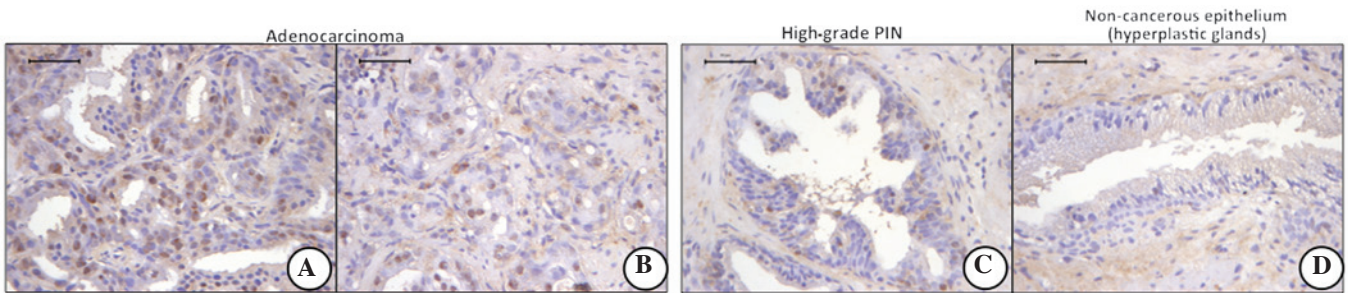
Figure 8. HIF-1 \alpha immunohistochemistry in ADC, high-grade PIN and hyperplastic glands. The number of HIF-1 \alpha -positive nuclei of (A and B) ADCs was greater than in (C) high-grade PIN. The number of HIF-1 \alpha -positive nuclei of (B) ADCs with Gleason scores of >3+4 was larger than that of (A) ADCs with Gleason scores of <3+3. No positive cell nuclei for HIF-1 \alpha were identified in the hyperplastic glandular cells (magnification, x200; scale bars, 50 \mu m). ADC, adenocarcinoma; HIF-1 \alpha , hypoxia-inducible factor-1 \alpha .; PIN, prostate intraepithelial neoplasia.
