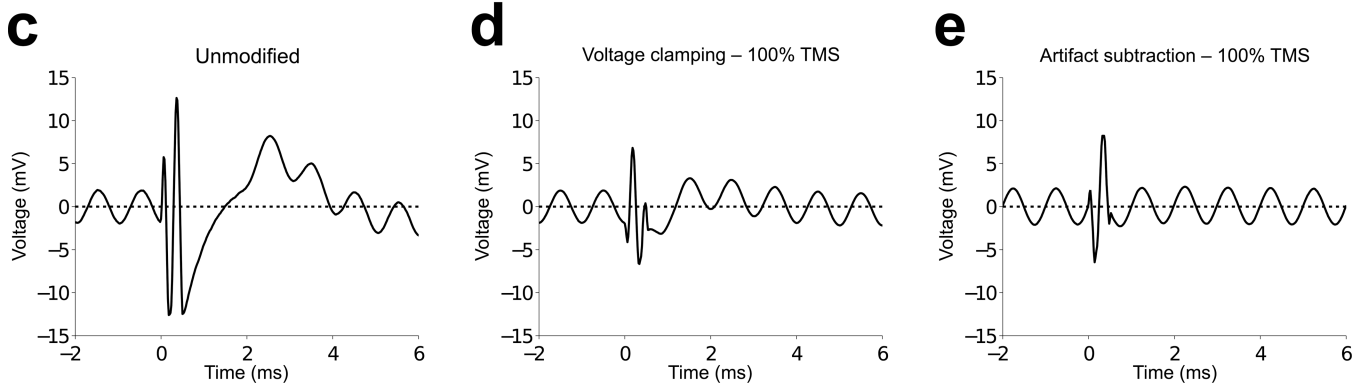
Figure 2. Voltage artifact reduction strategies. (a) Initial voltage clamping scheme modified from a BAK Electronics Model A-1 recording system. Based on an estimate of maximal neuronal signal amplitude of 100 \mu V, a gain of 10,000X can be implemented without clipping the neuronal signal, for an amplified neuronal signal of 1 V. (b) Voltage artifact subtraction behind front-end amplifier. A sense coil near the TMS coil generates a similar artifact waveform as that detected in the recording electrode. The sense coil's artifact is scaled such that adding it to the signal from the electrode reduces the TMS artifact dramatically while leaving the neuronal signals unperturbed. The gain and polarity required for artifact scaling is dependent on the size of, and number of turns in, the sense coil, as well as its location and orientation relative to the TMS coil. The use of two rheostats with variable turns functions as separate coarse and fine adjusts for artifact scaling. (c) TMS caused distortion and loss of signal in the unmodified recording electronics immediately following the stimulus pulse. (d) Voltage clamping diodes prevented saturation of recording amplifiers by the TMS artifact,
