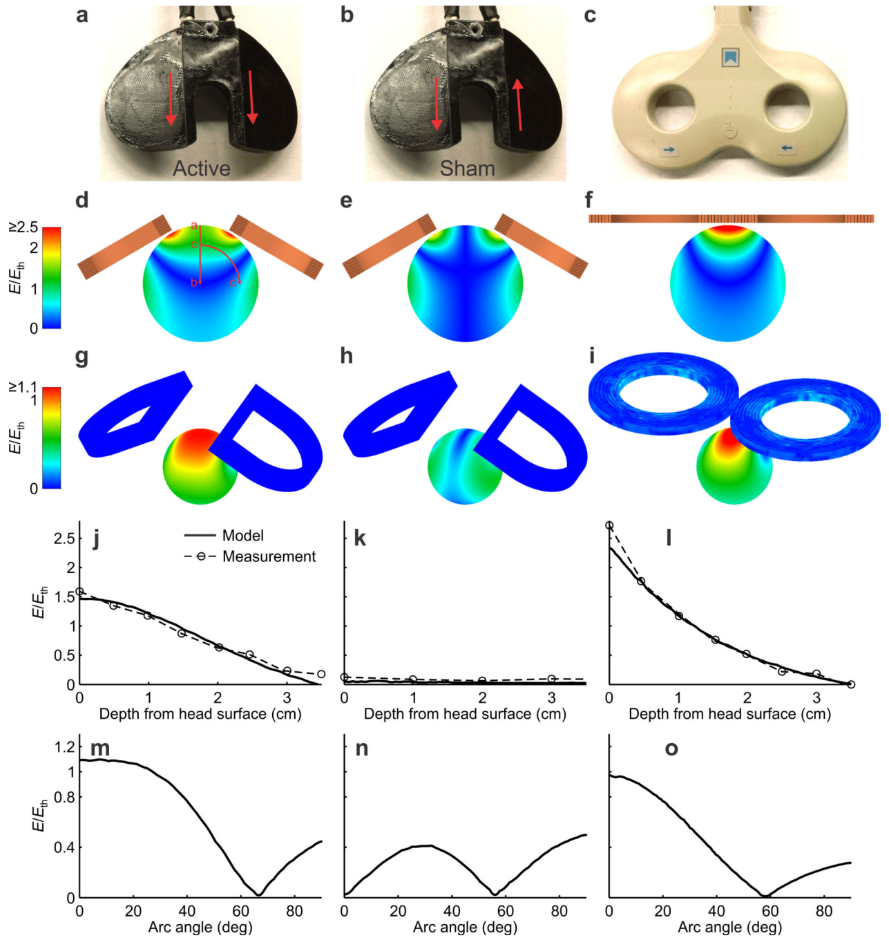
Figure 1. Models and measurements of the chamber centric coil compared with the Magstim 70 mm butterfly coil at 100% stimulator output (Magstim Rapid 2 base unit). (a) Chamber centric coil in Active mode. In this configuration, current directions along the central segments of the coil are parallel, as indicated by the red arrows. (b) Chamber centric coil in Sham mode. Current directions along the central segments of the coil are antiparallel. (c) Magstim 70 mm butterfly coil, to scale with the chamber centric coil. In the remaining panels, the three illustrations in each row conform to the coils and modes of (a)-(c), i.e. left panel is always
