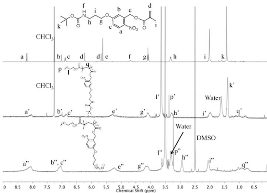
Fig. 2. 1 H NMR spectra of Boc-APNBMA monomer (top) in CDCl 3 , mPEG- b -P(Boc-APNBMA) n (middle) in CDCl 3 , and mPEG- b -P(APNBMA•HCl) n (bottom) in DMSO- d 6 . Letters with a single prime (') indicate resonances from the protected BCP and letters with a double prime (") indicate resonances from mPEG- b -P(APNBMA•HCl) n .
