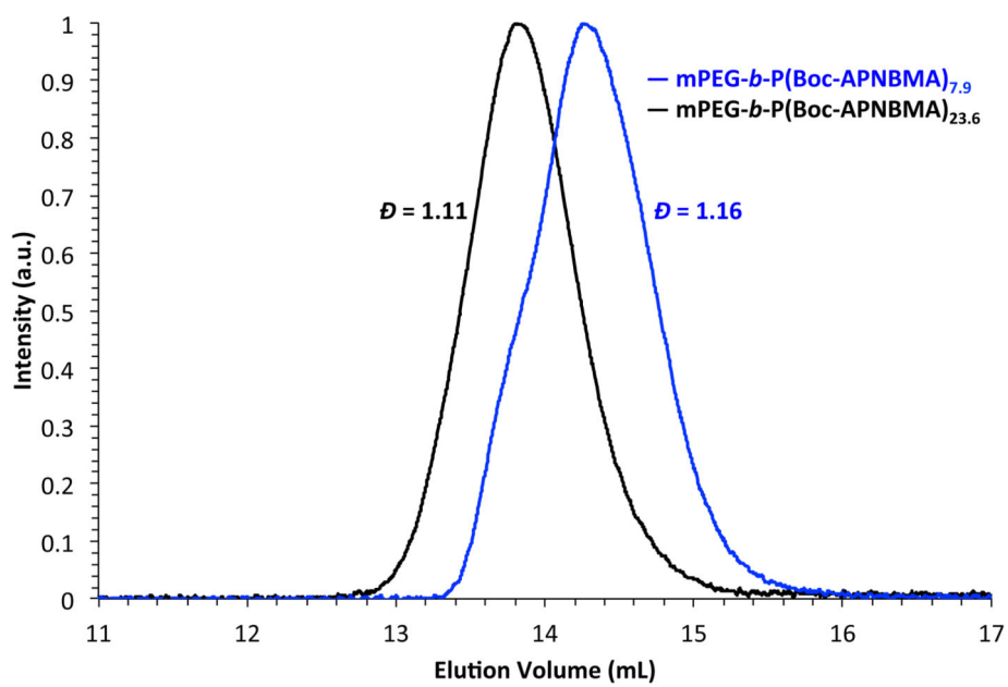
Fig. 1. Size exclusion chromatograms of \text{mPEG-}b\text{-P(Boc-APNBMA)}_n .
