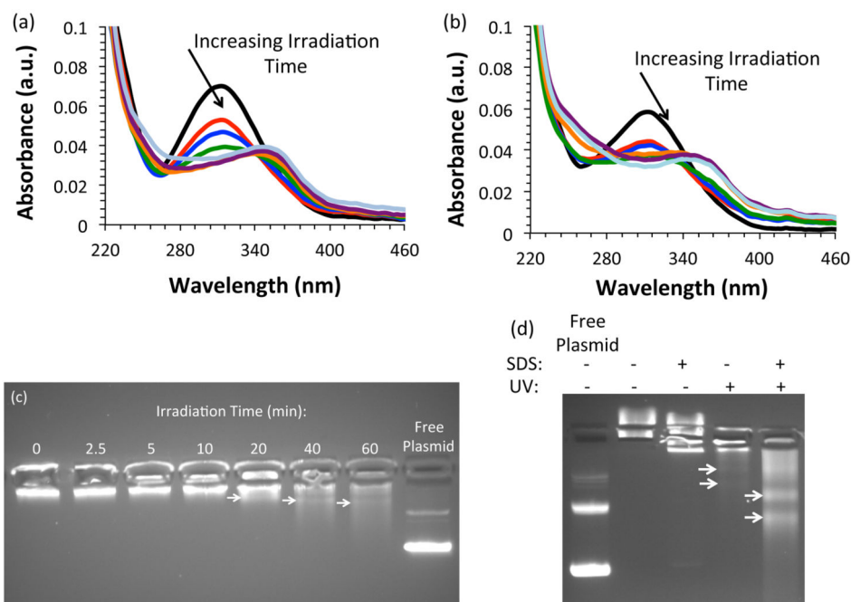
Fig. 5. UV-visible spectroscopy of (a) mPEG- b -P(APNBMA•HCl) 7.9 following exposure to 365 nm light at 200 W/m 2 for 0 (black), 2.5 (red), 5 (blue), 10 (green), 20 (orange), 40 (purple), and 60 (teal) min; and (b) pDNA/mPEG- b -P(APNBMA•HCl) 7.9 polyplexes following exposure to 200 W/m 2 for 0 (black), 2.5 (red), 5 (blue), 10 (green), 20 (orange), 40 (purple), and 60 (teal) min. Gel electrophoresis of pDNA/mPEG- b -P(APNBMA•HCl) 7.9 polyplexes following exposure to (c) UV at varying irradiation times, and (d) a combination of SDS surfactant at a sulfate/phosphate (S/P) ratio of 20 and subsequent UV irradiation. The arrows in (c) and (d) indicate the location of higher intensity fluorescence bands, which potentially correlate to supercoiled DNA or open circular DNA that is interacting with photocleavage fragments and hence prohibited from migrating as free pDNA. The free pDNA (“Free Plasmid”) in (c) and (d) was irradiated with UV light to demonstrate the lack of UV-mediated crosslinking.
