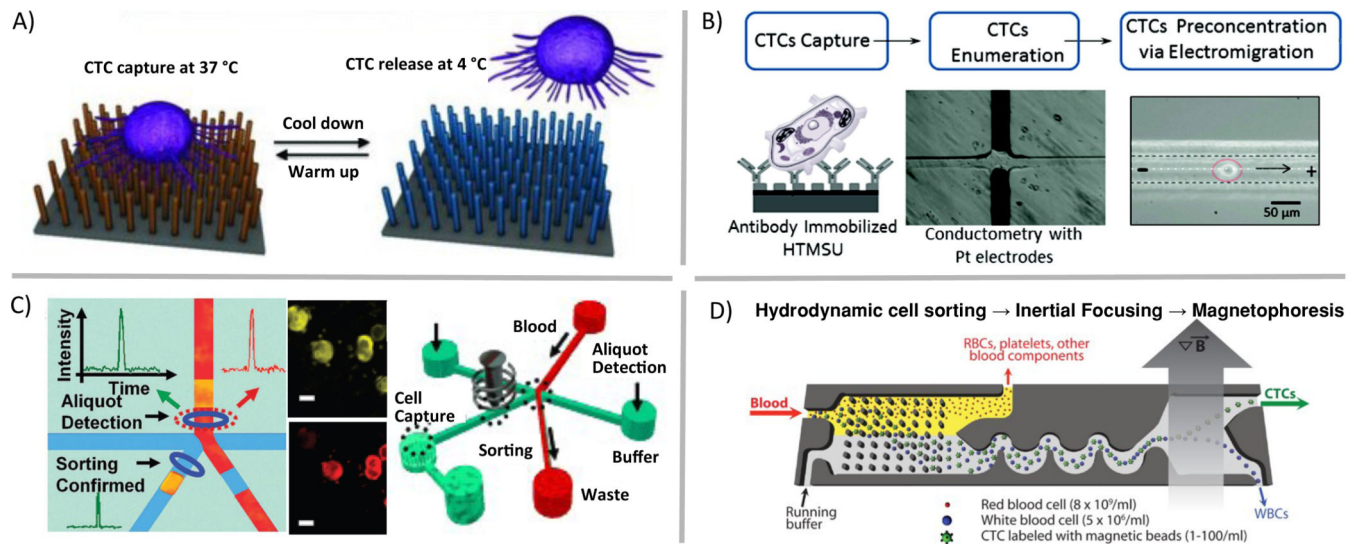
Fig. 2. Microfluidic enrichment of rare cells. Circulating tumor cells (CTCs) can be enriched from whole blood using a variety of techniques including A) nanostructure and antibody-based reversible surface capture [reprinted (adapted) with permission from ref. 10. Copyright 2013 Nature Publishing Group], B) affinity capture combined with electrokinetic enrichment [reprinted (adapted) with permission from ref. 11. Copyright 2011 American Chemical Society], C) microfluidic aliquot sorting of target cells combined with on-chip filtration [reprinted (adapted) with permission from ref. 12. Copyright 2012 Angewandte Chemie, International Edition], and D) combined hydrodynamic-magnetic methods [reprinted (adapted) with permission from ref. 13. Copyright 2013 AAAS].
