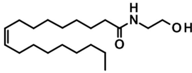
Oleoylethanolamide (OEA)
