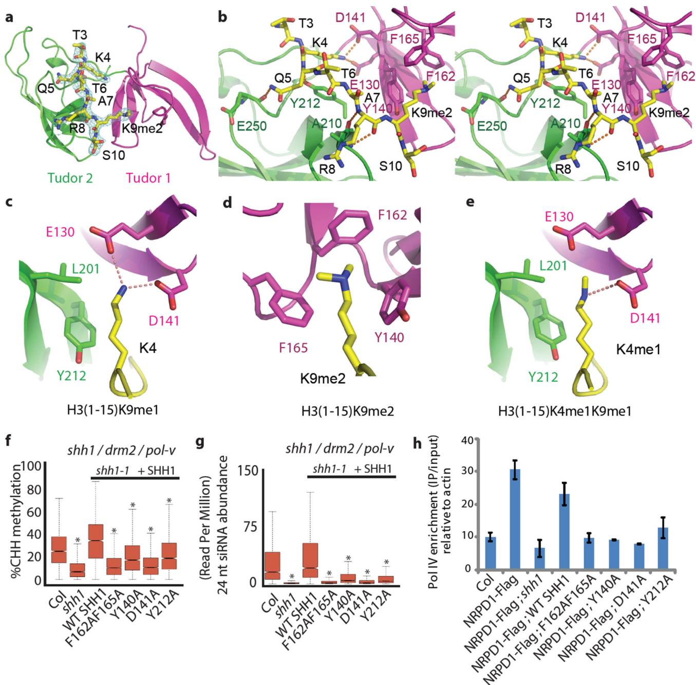
Figure 4. Structural basis for recognition of H3(1–15)K9me2 peptide by the SHH1 SAWADEE domain and the functional impact of mutations of residues lining the K4 and K9me2 pockets a , Overall structure of the H3(1–15)K9me2-SAWADEE complex with the SAWADEE domain as a ribbon diagram and the peptide as a stick representation. The simulated annealing composite omit map at 1\sigma level of the bound peptide is also shown. b , Stereo view highlighting the intermolecular interactions between the SAWADEE domain and the bound peptide. Intermolecular hydrogen-bonding interactions are designated by dashed red lines. c , d and e , Close-up views of H3 lysine residues in their respective binding pockets. f and g , Boxplots of genome-wide % CHH methylation and siRNA levels in wild-type, shh1
