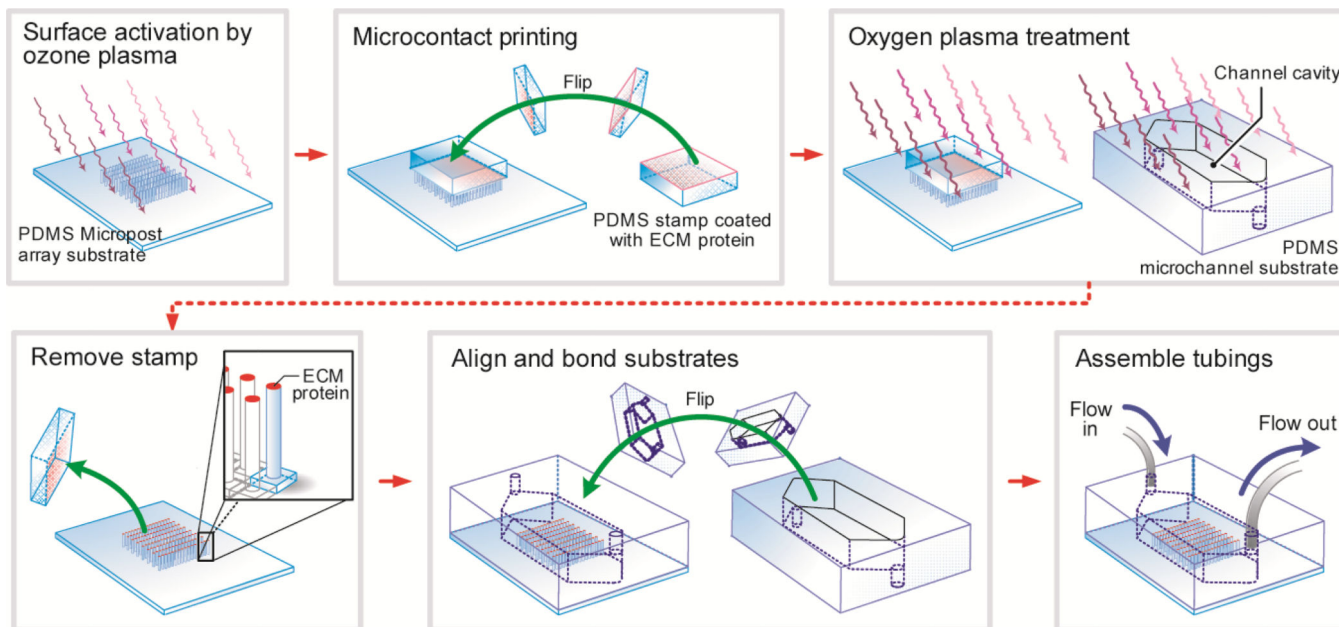
Figure 1. Schematic of the fabrication process for the \mu PAC device. The \mu PAC device was fabricated using a soft-lithography compatible fabrication technique, and it contained a rectangular microfluidic channel embedded with a hexagonally arranged PDMS micropost array on the bottom surface of the microfluidic channel. Using microcontact printing, the tops of the PDMS microposts were selectively coated with adhesive ECM proteins for cell seeding.
