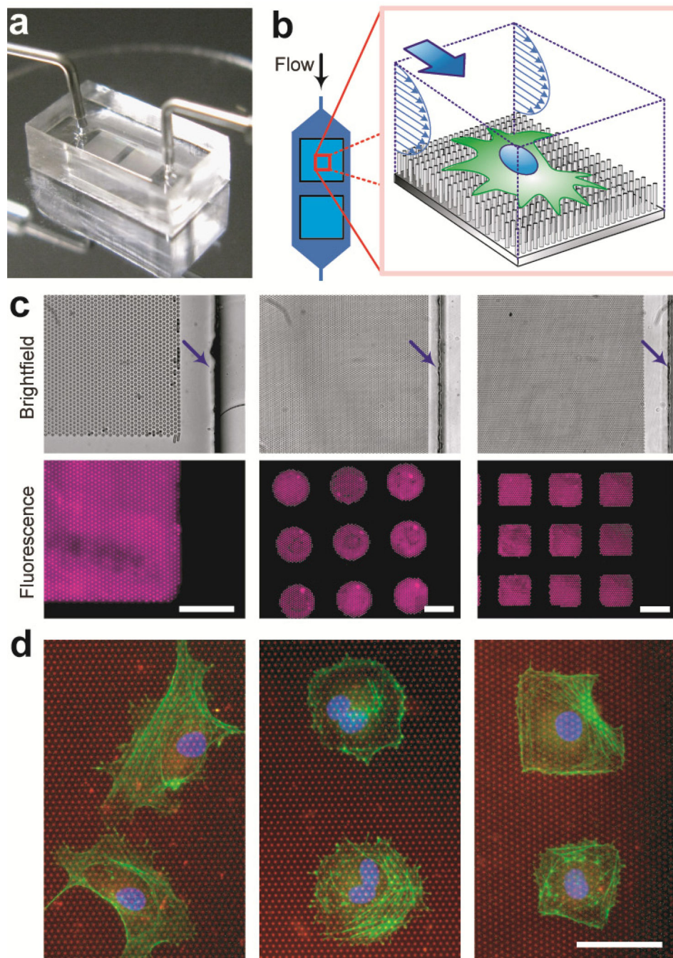
Figure 2. The \mu PAC device with the microfluidic channel embedded with the PDMS micropost array coated with different patterns of adhesive ECM molecules. (a) The \mu PAC device (dimensions: 10 mm ( l ) \times 5 mm ( w ) \times 4 mm ( h )) connected with external tubing for the fluid supply and control. (b) Cartoon of a single cell plated on the PDMS microposts and the cell culture medium flowing continuously along the microfluidic channel to exert fluid shear stress on the cell. (c) Brightfield microscopic images ( top row ) and corresponding fluorescence images ( bottom row ) of the PDMS micropost array coated with different
