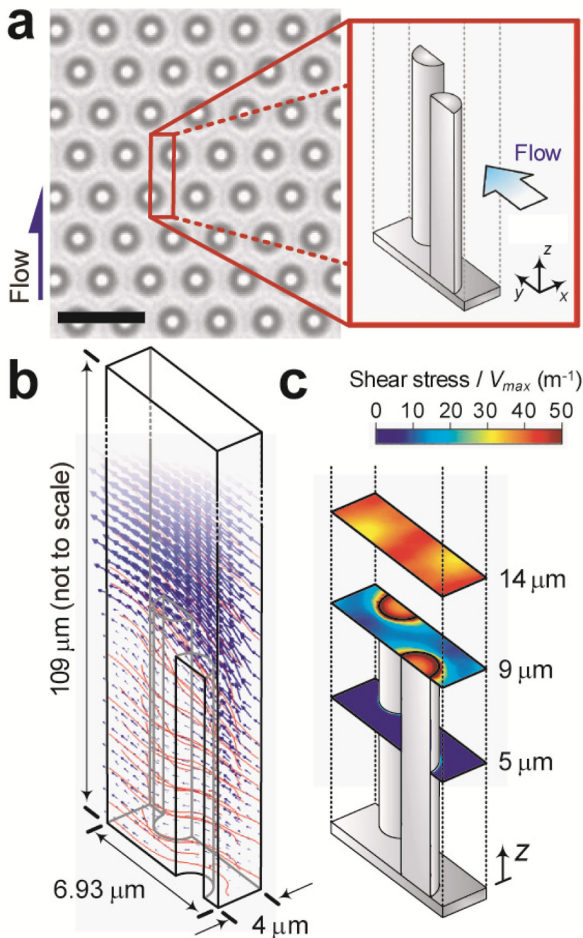
Figure 3. Simulation of flow characteristics in the microfluidic channel of the \mu PAC device. (a) Brightfield microscopic image of the PDMS micropost array embedded at the bottom of the microfluidic channel of the \mu PAC device. The inset shows the repeating geometrical unit used for flow simulation. Scale bar, 6\ \mu\text{m} . (b) Simulation results of flow velocity ( blue arrows ) and streamlines ( red curves ) around the PDMS microposts. (c) Colorimetric maps showing magnitudes of the shear stress at different horizontal planes along the height of the PDMS microposts as indicated.
