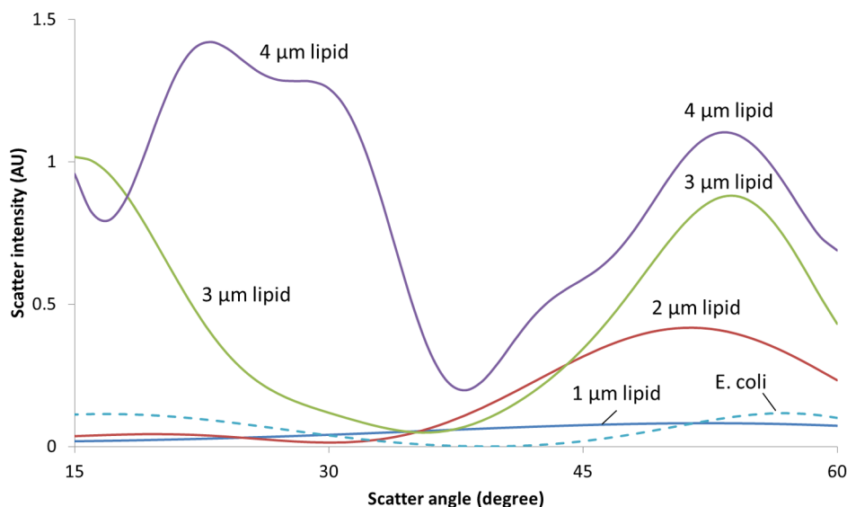
Figure 7 | Mie scatter simulations for lipid particles and E. coli .
