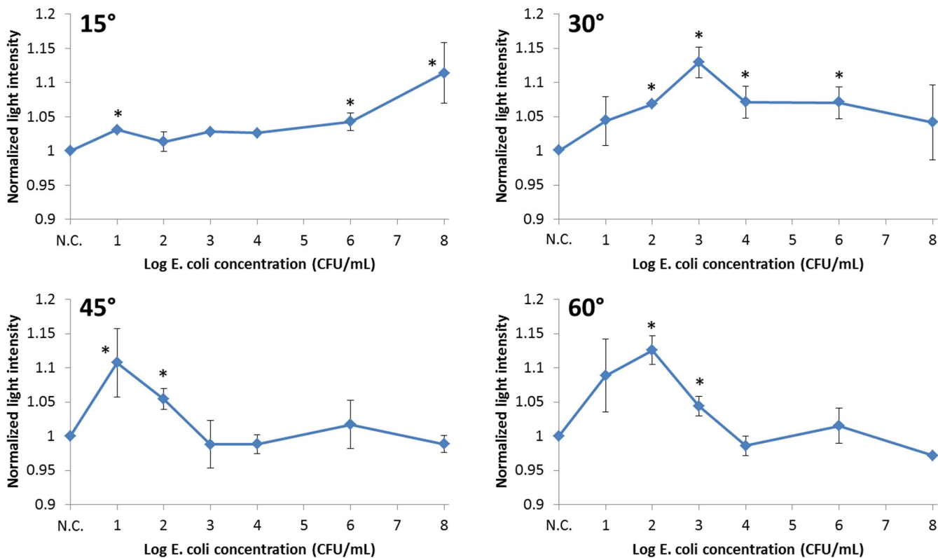
Figure 3 | Normalized scatter light intensities plotted against the log concentrations of E. coli on ground beef. Error bars represent standard errors. The scatter detection angle was 15°, 30°, 45° and 60°. Each data point represents the mean of three replicates (each measured from different locations on a ground beef sample). A new ground beef sample was used for each E. coli concentration. Stars (*) represent the data points that are significantly different from the negative control, with p < 0.05 (two-sample t-tests).
