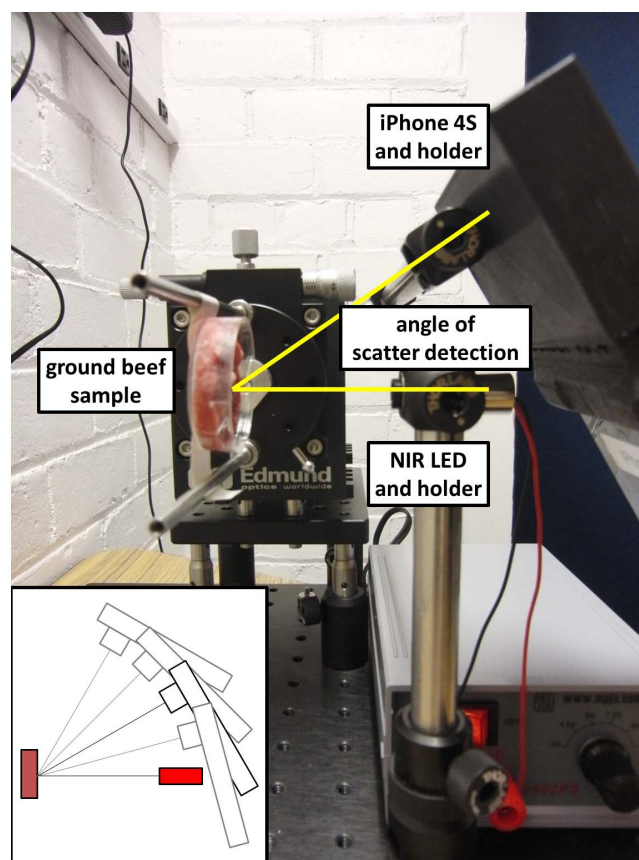
Figure 1 | The benchtop system consists of an iPhone 4S and its holder, an NIR LED and its holder, and a ground beef sample and its holder. The angle of scatter detection refers to the angle between the iPhone camera and the NIR LED light source.
