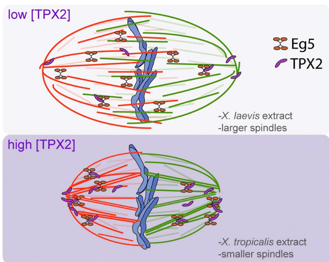
Figure 5. Model of TPX2 regulation of spindle size and MT distribution via Eg5. MTs with plus ends to the right are red, whereas MTs with the opposite orientation are green. An increase in TPX2 (purple) concentration recruits more Eg5 (orange) to the spindle poles, reducing the extent of MT overlap and increasing MT cross-linking at spindle poles, thereby causing spindle length to decrease.
