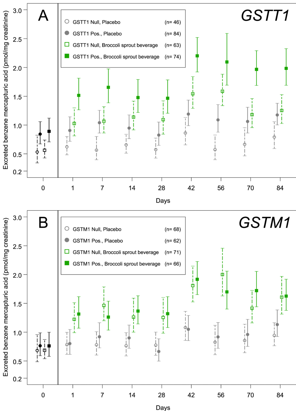
Figure 3. Effect of GSTM1 and GSTT1 genotypes on urinary excretion of benzene-mercapturic acid. Distributions of benzene-mercapturic acid levels (geometric means and 95% confidence intervals) in participants either null or positive for the GSTT1 gene (panel A) or the GSTM1 gene (panel B) by assignment group (placebo or treated and day of study). Bars highlighted in green indicate those receiving the broccoli beverage. Open symbols represent medians for the participants null for the genotype and solid symbols indicate the geometric means of those who were positive.
