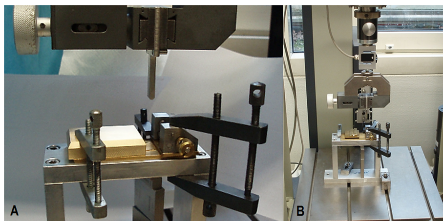
Figure 3 Three-point bending/breaking test set-up with the two different platform options. A) The three-point bending/breaking device strapped into a ZWICK-testing machine type Z2020/TND (ZWICK-/Roell, Ulm, Germany) with a solid aluminum block as contact point for the distal diaphyseal tibia. B) Overview of the ZWICK-testing machine and the three-point bending/breaking device with the mobile, ball-mounted platform as contact point for the distal diaphyseal tibia.
