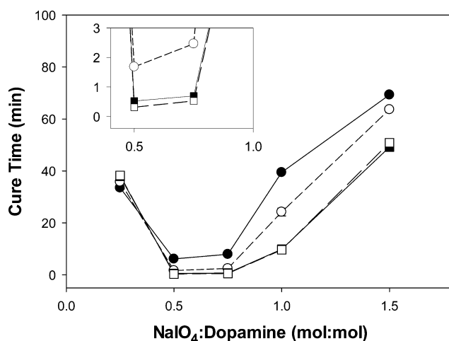
Figure 1. Cure time of PEG-D as a function of \text{NaIO}_4/\text{dopamine} molar ratio for hydrogels formulated with precursor solutions adjusted to a pH of 5.7 (●), 6.7 (○), 7.4 (■), and 8.0 (□). The inset enlarges the curing time results at a \text{NaIO}_4/\text{dopamine} molar ratio between 0.5 and 1.
