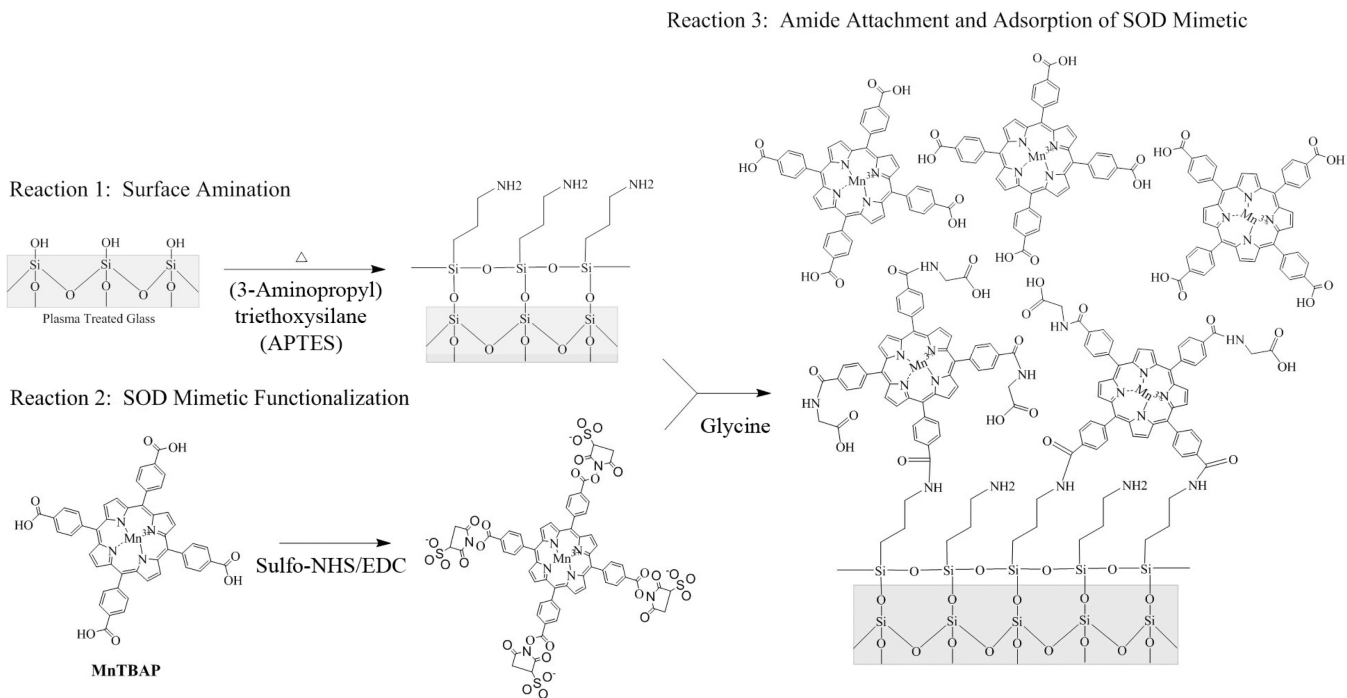
Figure 1. Reaction scheme for synthesis of MnTBAP modified glass surfaces.
