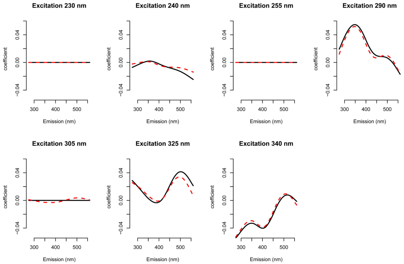
Figure 4. Estimated coefficient functions for the sugar data when using the standard functional group lasso with penalty (3) (dashed red) or the adaptive version (5) with adaptive w_j (solid black).
