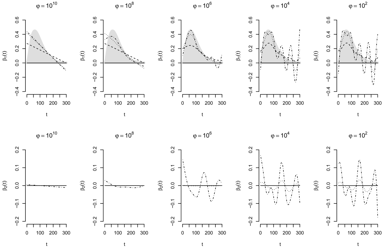
Figure 1. Fitting results for the functional group lasso for \lambda \in \{10^3, 10^2, 10^1, 10^0\} (solid, dashed, dotted, dashed/dotted, respectively) and \phi \in \{10^{10}, 10^8, 10^6, 10^4, 10^2\} on a simulated dataset with two functional covariates but only the first one being relevant; the first row corresponds to the first covariate (with the true coefficient function shaded in grey), the second row to the actually irrelevant signals.
