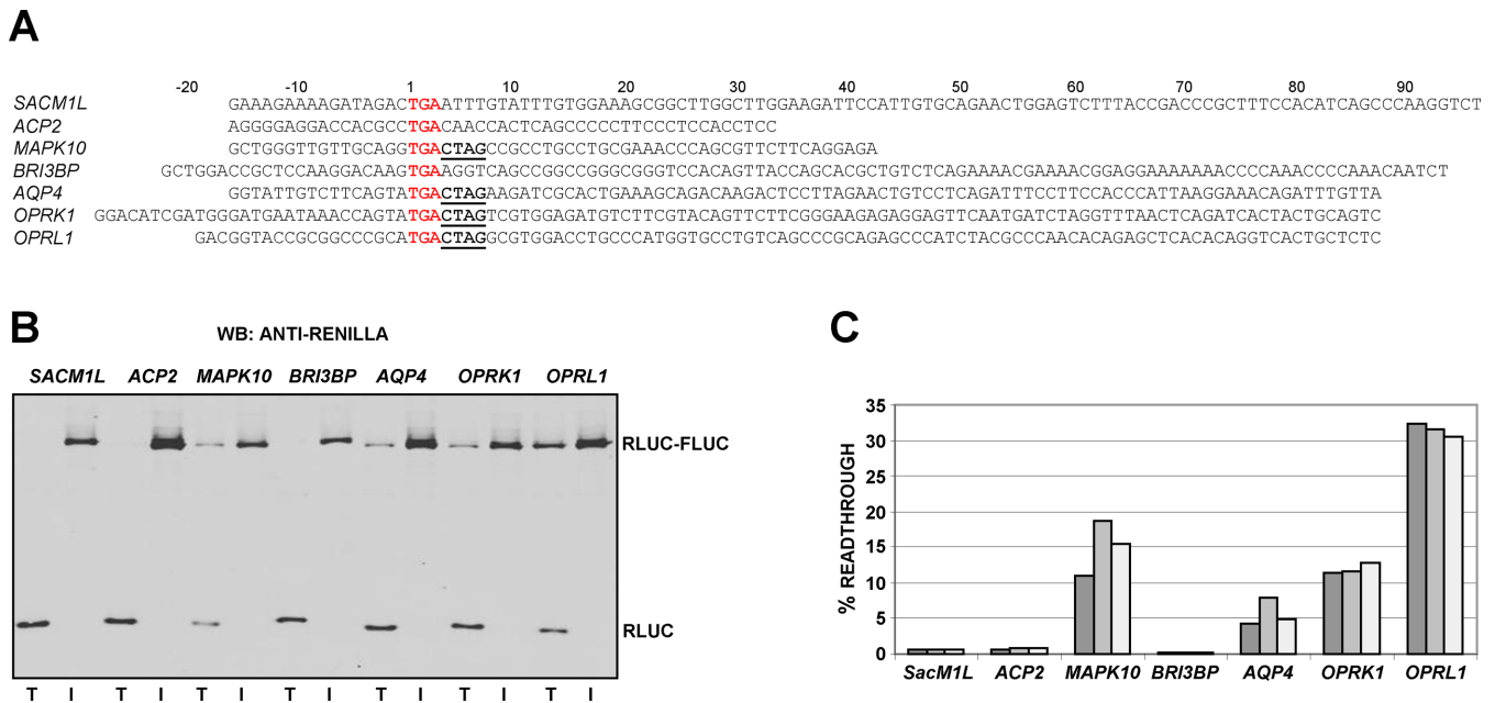
Figure 2. (A) Sequence boundaries of seven readthrough candidates cloned into a dual-luciferase plasmid. Main ORF stop codons are in red font and the conserved CTAG motif is highlighted in bold and underlined. Plasmids were transfected into HEK-293T cells and 24 hr later lysates analysed for readthrough by both western blotting with anti-Renilla (B) and dual-luciferase assay to determine readthrough efficiencies (C). For (B) each TGG in-frame control (I) is adjacent to its respective test (T) construct. For (C) readthrough efficiencies were calculated as the ratio of test construct luciferase activity to its TGG in-frame control from three independent experiments.
