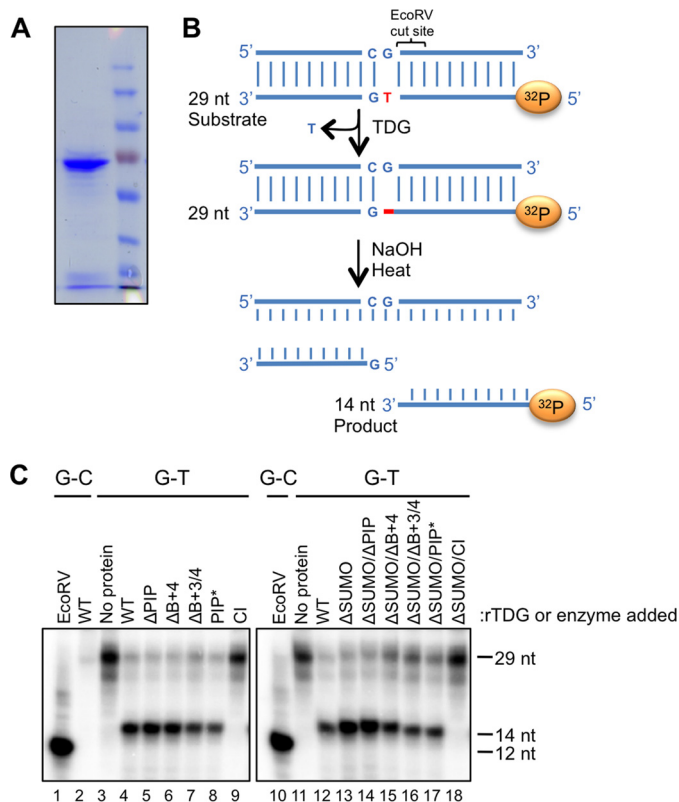
FIGURE 3. Characterization of Xenopus TDG protein. A , native TDG from E. coli was purified and analyzed by SDS-PAGE and Coomassie Blue staining. B , schematic of the base release assay used to monitor TDG activity. Double-stranded DNA (29 bp) containing a site-specific G-T mismatch is 5'-radiolabeled on the DNA strand containing the thymine of the mismatch. TDG activity generates an abasic site, and subsequent treatment with sodium hydroxide and heat leads to hydrolysis of the backbone at the abasic site. TDG activity is measured as the appearance of a 14-nt product. As a control, the oligonucleotide was treated with EcoRI, which cleaves adjacent to the G-T mismatch in the fully complementary duplex to generate a 12-nt product. C , recombinant wild type TDG and all TDG mutants used in this work, except the catalytically inactive form (CI), are active in the base release assay diagramed in B . Detailed descriptions of these mutants can be found upon their first experimental usage in Figs. 5 and 6. The concentration of TDG in all reactions was 100 nM, and the DNA concentration was 50 nM. Strand cleavage was measured using a 15% polyacrylamide gel.
