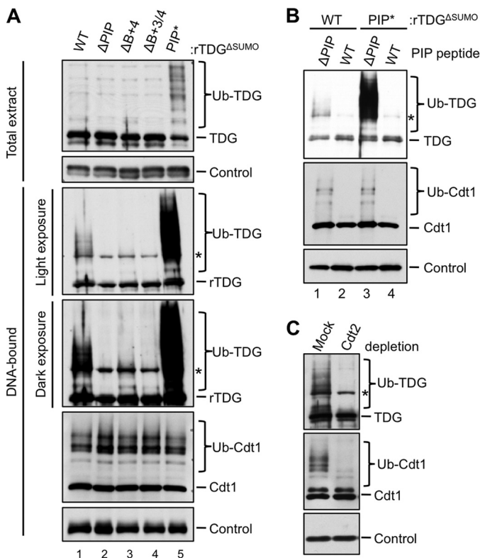
FIGURE 8. TDG is ubiquitylated on chromatin in a PIP box-, PCNA-, and Cdt2-dependent manner. A , the effect of different TDG mutations on its ubiquitylation. The indicated TDG proteins (described in the legend to Fig. 6B) were added to egg extract containing methyl ubiquitin (2 mg/ml) before the addition of 50 ng/μl MMS-damaged linear DNA immobilized on magnetic beads. The beads were recovered, and associated TDG was monitored via immunoblotting with anti-TDG antibodies. TDG in total extract is also shown. B , the addition of a PIP box competitor peptide abolishes ubiquitylation of both TDG ΔSUMO and TDG ΔSUMO/PIP* . p21 peptide was added to egg extract as in Fig. 6A, and TDG ubiquitylation was monitored as in Fig. 8A. C , depletion of Cdt2 eliminates ubiquitylation of DNA-bound TDG ΔSUMO . Extract was mock-depleted or immunodepleted of Cdt2 and supplemented with TDG, methyl ubiquitin, and linear DNA. TDG ubiquitylation was monitored as in Fig. 8A. In all panels, the asterisk indicates two overlapping bands: specific signal (ubiquitylated TDG) and a nonspecific signal. The loading controls for each panel are as follows: Orc2 ( A , DNA-bound), nonspecific band detected by TDG antibody ( A , Total extract), RPA-14 ( B ), and PCNA ( C ).
