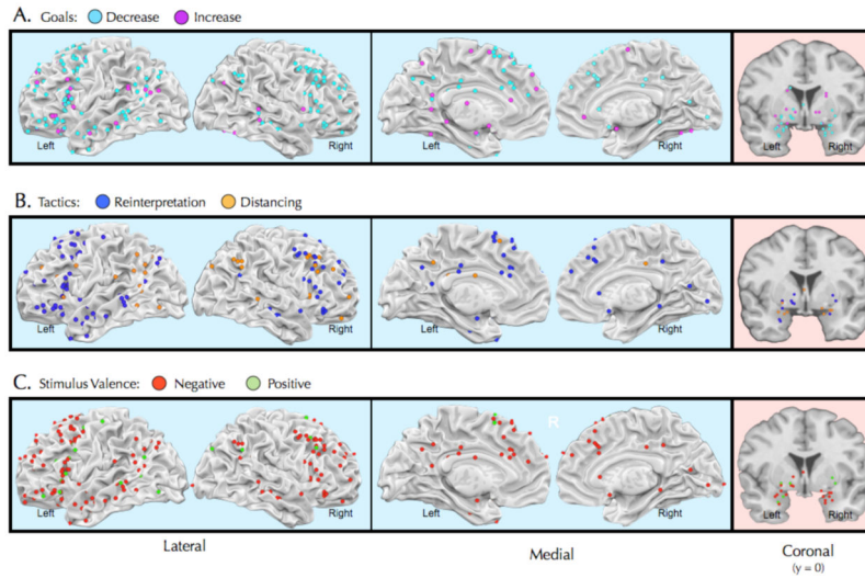
Figure 3. Plots of activation foci from the 43 studies of reappraisal described in the text and Table. A. Plots of foci as a function of the goals to decrease or increase emotion. B. Plots of foci as a function of the specific reappraisal tactics used – either reinterpreting the meaning of events depicted in stimuli or actively changing one’s psychological distance from them. C. Plots of foci as a function of the valence of the stimuli eliciting the emotions that participants attempted to regulate. Blue boxes illustrate regions that are purported to support reappraisal (increase>look and decrease>look contrasts). Pink boxes illustrate regions that are purported to be modulated by reappraisal (look>decrease and increase>look contrasts; for clarity only foci falling within the boundaries of the amygdala and striatum are shown).
