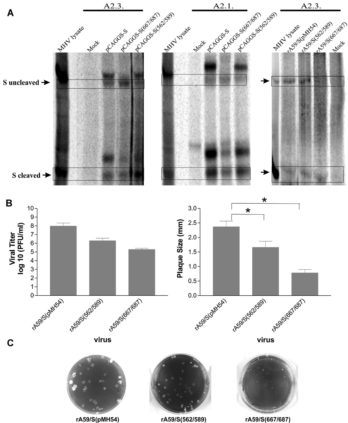
Fig. 5. The effect of the replaced paired residues T562L/T589L and S667 T/D687Y on viral replication and reproduction. (A) Immunoprecipitation of 293 T cells transfected with the expression vector pCAGGS-S or the expression vector encoding the S protein with the paired replaces residues in positions 562/589 and 667/687 of the spike protein (pCAGGS-S (562/589) and pCAGGS-S (667/687), respectively). The cells were metabolically labeled with [ 35 S]-methionine and cysteine for eight hours in 37 °C and the lysate was precipitated with monoclonal anti-S antibodies A2.1 and A2.3. S uncleaved denotes the 180 kDa spike protein and S cleaved represents the 90 kDa cleaved S1 and S2 subunits. (B) Mean viral titers and plaque diameters of the recombinant viruses rA59/S (562/589), rA59/S (667/687) and rA59/S (pMH54) expressing the mutated and the native spike protein, correspondingly. Error bars represent the standard deviation from the mean. (C) Plaque morphologies of the recombinant viruses expressing the native and the mutated spike proteins.
