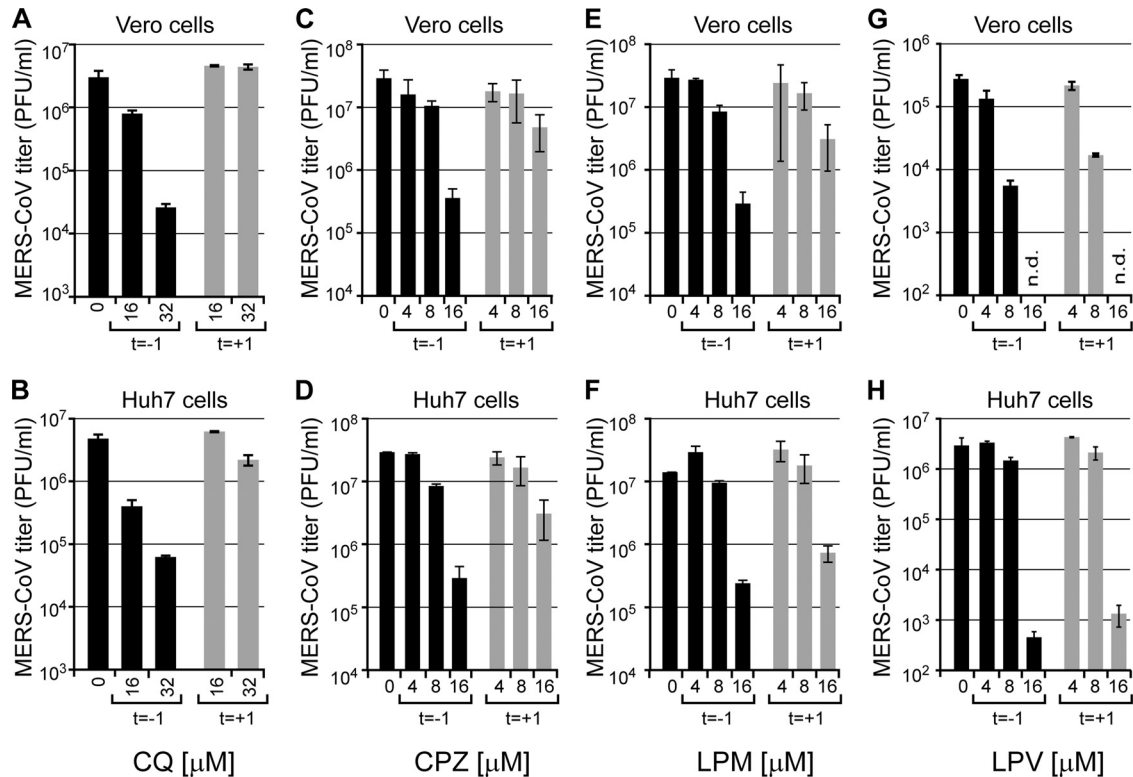
FIG 4 Chloroquine, chlorpromazine, loperamide, and lopinavir affect various stages of the MERS-CoV replication cycle. Vero (A, C, E, G) and Huh7 cells (B, D, F, H) were infected with MERS-CoV isolate EMC/2012 (MOI, 1). At t = -1 or +1 , the indicated concentrations of CQ (A, B), CPZ (C, D), LPM (E, F), and LPV (G, H) were added, and virus titers in the culture supernatant ( n = 4 ; averages and SDs are shown) were determined at 24 h p.i. using plaque assays; n.d., not detected.
