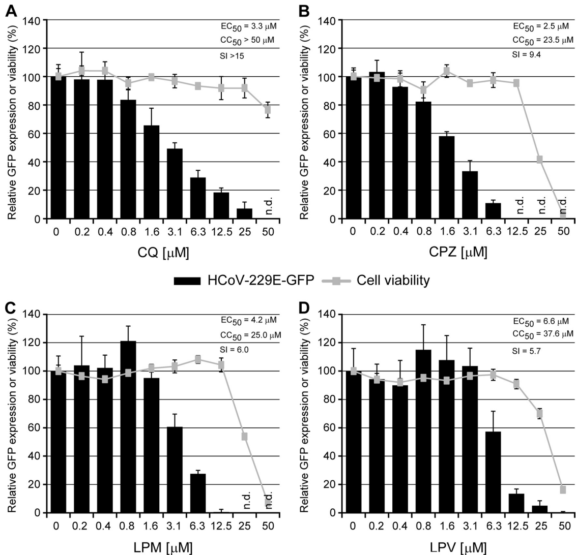
FIG 3 HCoV-229E-GFP replication is inhibited by low-micromolar amounts of chloroquine, chlorpromazine, loperamide, and lopinavir. Huh7 cells in 96-well plates were infected with HCoV-229E-GFP (MOI, 5) in the presence of 0 to 50 \mu\text{M} CQ (A), CPZ (B), LPM (C), or LPV (D). Compounds were given at t of -1 and remained present during infection. Cells were fixed at 24 h p.i., and GFP reporter gene expression was measured and normalized to the signal in control cells (100%; black bars), which were treated with the solvent used for the various compounds. The effect of compound treatment on the viability of mock-infected Huh7 cells, compared with solvent-treated control cells, was determined by using an MTS assay (gray lines). Graphs show the results (average and SD) of a representative quadruplicate experiment. All experiments were repeated at least twice; n.d., not detected.
