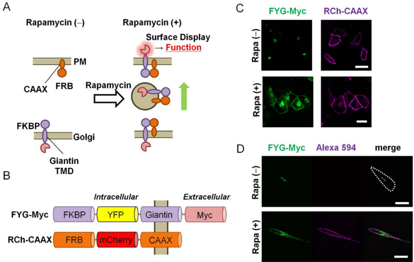
Fig. 1. DISplay, a chemically induced, cell-surface engineering technique
