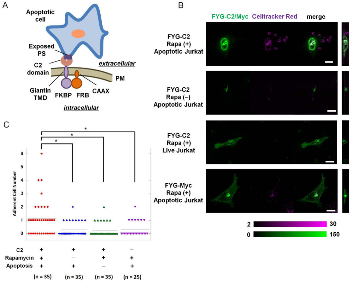
Fig. 2. Rapidly induced display of the C2 domain of MFG-E8 at the cell-surface stimulates binding to apoptotic cells
