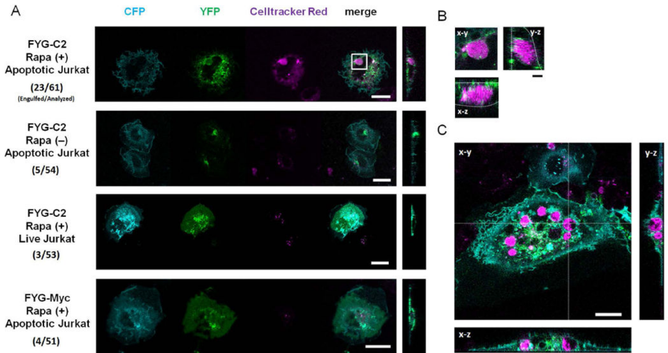
Fig. 3. The rapidly induced display of the C2 domain of MFG-E8 at the cell-surface coupled with the activation of intracellular Rac1 stimulates the engulfment of apoptotic cells (A) HeLa cells transfected with plasmids encoding CFP-Rac1 (CA), FRB-CFP-CAAX (RCh-CAAX), and either FYG-C2 or FYG-Myc were left untreated or were treated with 200 nM rapamycin for 60 min, and then were incubated for 12 hours in the presence of CellTracker Red–labeled apoptotic or live Jurkat cells before being analyzed by fluorescence microscopy. Signals from CFP, YFP, and CellTracker Red are presented in cyan, green, and magenta, respectively. Scale bar: 20 \mu m. Right: micrographs are y-z plane images of the merged fluorescence. The numbers of cells engulfed versus those analyzed are shown. Statistical analysis is summarized in Table 1 and table S1. (B) Magnified view of an engulfed Jurkat cell indicated by the white square in (A). Right and bottom micrographs indicate y-z and x-z plane images, respectively. White dotted lines indicate the cell periphery of the HeLa cells. Images in (A) and (B) are representative of at least 51 cells from two independent experiments. Scale bar: 4 \mu m. (C) Representative fluorescence images of COS7 cells (cyan) with engulfed apoptotic cells (magenta) shown in three confocal planes (x-y, x-z, and y-z). The COS7 cells were transfected with plasmids encoding CFP-Rac1 (CA), FRB-CFP-CAAX (RCh-CAAX), and FYG-C2, treated with 200 nM rapamycin for 60 min, and incubated for 12 hours in the presence of apoptotic Jurkat cells labeled with CellTracker Red. Images in (C) are representative of 54 cells from two independent experiments. Statistical analysis is summarized in tables S2 and S3. Scale bar, 20 \mu m.
