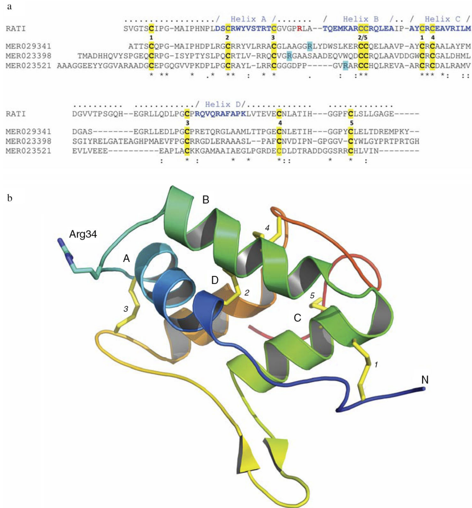
Fig. 2. Rice-derived proteins inhibiting gingipains. (a) Crystal structure-guided alignment of a bifunctional inhibitor of alpha-amylase and trypsin (RATI) from ragi seeds (Indian finger millet, Eleusine coracana Gaertneri) (MER018247) and rice-derived proteins inhibiting gingipains: alpha-amylase/trypsin inhibitor (MER029341), seed allergic protein RA17 precursor (MER023398) and plant lipid transfer/seed storage/trypsin-alpha amylase inhibitor domain containing protein (MER023521). Conserved cysteine residues and arrangement of disulfide bridges are highlighted yellow and induced by the identical digit between the RATI and MER029341 sequences, respectively. Amino acid residues forming alpha-helices (A, B, C, and D) are in bold blue font and the reactive site loop is located between helices A and B. The reactive site Arg residue in the RATI structure is in the bold red font. Arg residues in rice proteins, which may be recognized by Rgps as the P1 residues in the inhibitory reaction are highlighted turquoise. ‘-’ gaps introduced into sequences to facilitate the alignment using the ClustalW program ( http://embnet.vital-it.ch/software/ClustalW.html ). (b) The crystal structure of RATI (PDB database: 1B1U). The reactive site residue Arg34 is shown in ball-and-stick representation in purple.
