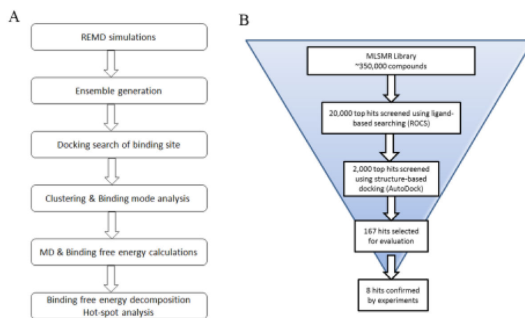
Figure 2. (A) Stepwise binding mode analysis combining an unbiased docking search, clustering analysis, MD simulation and binding free energy calculations to probe the binding interaction of BoNT/A inhibitors. (B) Flowchart of the virtual screening protocol.
