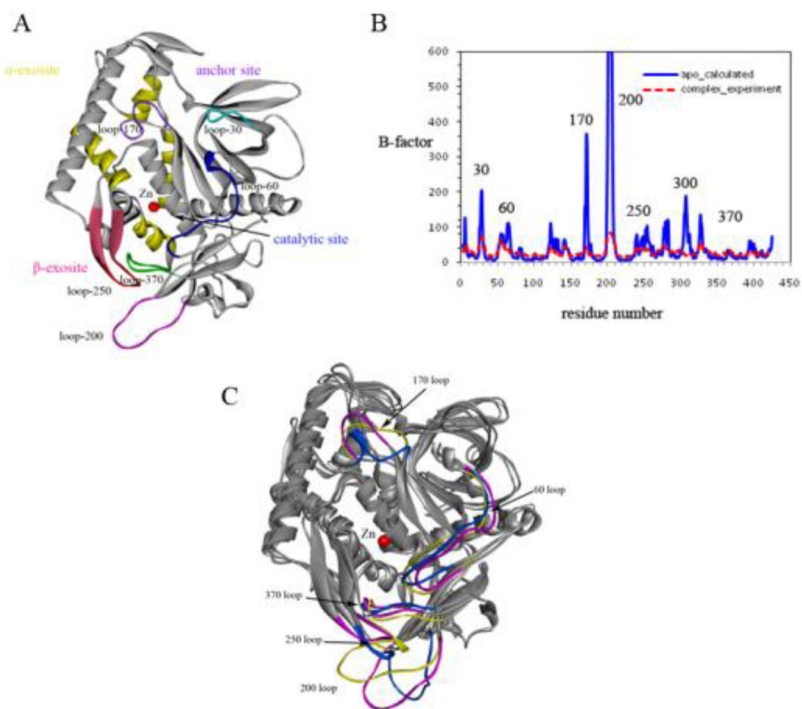
Figure 3. (A) Structure of the BoNT/A LC catalytic domain in ribbon representation. The catalytic binding site with Zn located at the center (red), the \alpha -exosite (yellow), the \beta -exosite sheet (magenta), the anchor site and other loops surrounding these binding sites are shown. (B) Calculated B-factors from MD simulations in comparison with the experimental B-factors. (C) Conformations of BoNT/A observed from essential dynamic analysis. The first essential mode is associated with loops 200, 250, and 370 at the \beta -exosite, while the second dynamical mode is found with loops 60 and 170 surrounding the active site.
