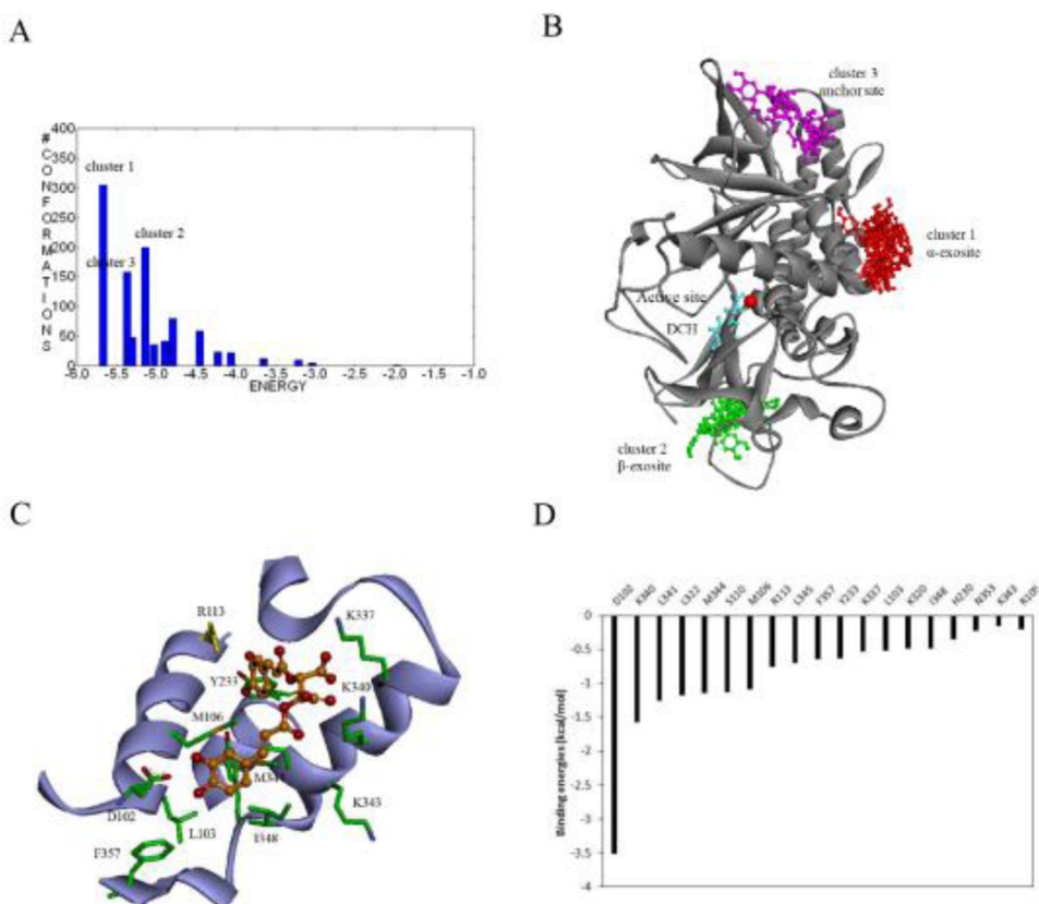
Figure 4. (A) Cluster analysis of binding modes of D-chicoric acid docked to BoNT/A using AutoDock 4.2. Members of docked poses in the cluster are shown on the Y-axis. The X-axis shows the lowest docked score found in the cluster. (B) Three major clusters of D-chicoric acid bound to the \alpha -exosite (red), the \beta -exosite (green), and the anchor exosite (magenta) of BoNT/A. The DCH (cyan) interacts with Zn (red) at the active site. (C) Binding interaction of D-chicoric acid at the \alpha -exosite. The protein is shown as ribbons and key residues are shown as sticks. D-chicoric acid (dark yellow) is shown as ball and stick. (D) Hot-spot residues at the \alpha -exosite identified from the binding free energy decomposition.
