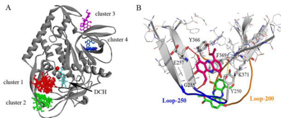
Figure 5. (A) Binding Clusters of lomofungin from SBMA clustering analysis. (B) Two binding modes of lomofungin bound at the \beta -exosite. Structure of BoNT/A is shown as ribbons. Lomofungin and key residues involved in binding (shown as sticks). Pairs of atoms involved in H-bonding are connected with dashed lines.
