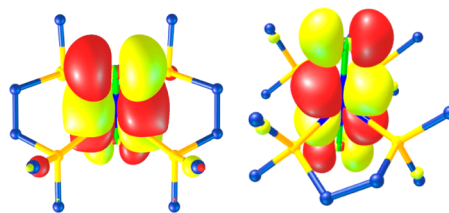
Figure 2. Degenerate SOMO comprising the ground state in [\text{W}^{\text{III}}\text{Cl}_2(\text{dppe})_2]^{1+} with \sim 72\% d_{x,yz} character.
