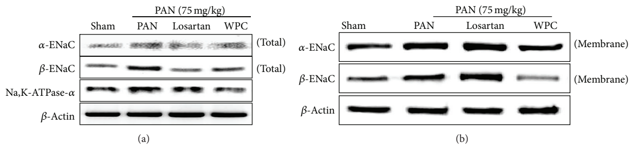
FIGURE 4: Effect of WPC on ENaC subunit and Na,K-ATPase- \alpha protein expression in PAN-induced nephrotic syndrome model. (a) The kidneys of medulla were total protein extracted determined by Western blot analysis. (b) The membrane fractions were extracted in medulla of kidneys and protein levels were determined by Western blot analysis.
