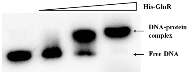
Figure 3. EMSA analysis of ald promoter with purified His-tagged GlnR. The promoter region of ald was amplified with primers aldbs_F2 and aldbs_A . Gamma- 32 P labeled DNA probe (0.04 pmol) was incubated with various amounts of purified GlnR (0 µg in lane 1, 0.4 µg in lane 2, 0.8 µg in lane 3 and 1.6 µg in lane 4). Two micrograms of sheared salmon sperm DNA was added to prevent nonspecific binding. doi:10.1371/journal.pone.0104811.g003
