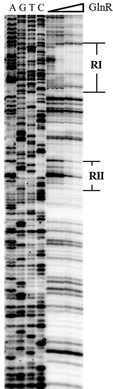
Figure 4. DNase I footprinting identification of the GlnR binding cis -element in ald promoter region. Different amounts of GlnR (0 µg in lane 1, 3 µg in lane 2, 6 µg in lane 3 and 9 µg in lane 4) were incubated with the labeled probes and DNA sequences protected by GlnR binding from DNase I cleavage were indicated (RI & RII). doi:10.1371/journal.pone.0104811.g004
