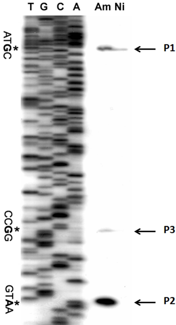
Figure 2. Identification of the transcription initiation sites (TISs) for ald . Total RNA was isolated from cultures in Bennet medium with different nitrogen sources, i.e., Am, 120 mM ammonium; Ni, 80 mM nitrate. TISs identified by the primer extension analysis were marked with asterisks and named as P1, P2 and P3, respectively. doi:10.1371/journal.pone.0104811.g002
