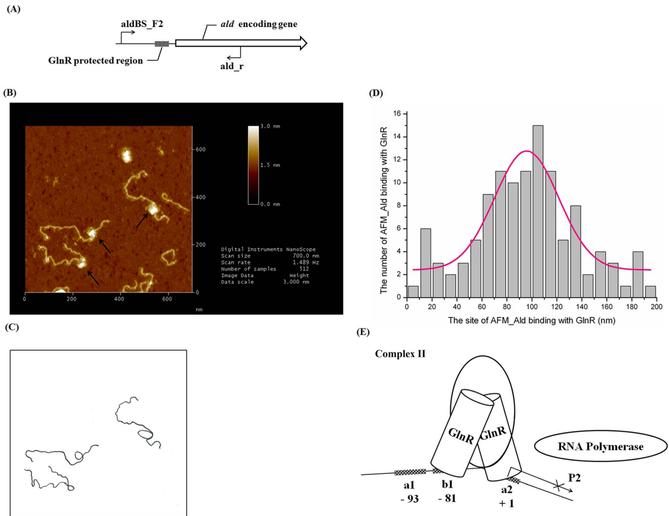
Figure 6. AFM analysis of the structural changes of ald promoter upon interaction with GlnR. (A) Schematic presentation of ald promoter used for AFM visualizing. (B) AFM images of fragment AFM_Ald with GlnR. Putative DNA loops were marked with black arrows. (C) Sketch of AFM_Ald fragments in Figure 6B, highlighting possible DNA loops. (D) Histogram of the distribution of GlnR binding sites on fragment AFM_Ald (n = 223 DNA molecules). The Gaussian centered 97 nm with a standard deviation of 42 nm. (E) Proposed mechanisms for GlnR-mediated negative regulation of ald transcription. GlnR finally binds b1 and a2 sites to form Complex II and blocks ald transcription initiated from aldP2 , which contributes the majority of ald transcripts under nitrogen-excess conditions. A DNA loop may occur during the process. The numbers labeled show their relative distance to aldP2 site.
