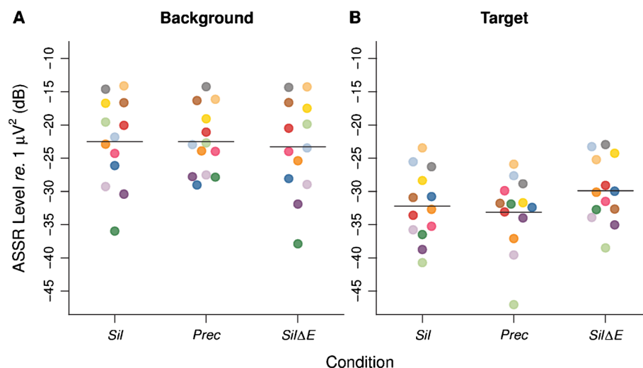
FIG. 3. A ASSR levels for the background components as a function of precursor type. B ASSR levels for the target component as a function of precursor type. Each colored point represents an individual listener. The color code is the same as in Figure 2. The horizontal segments represent the across-listener averages
