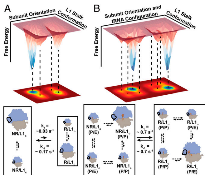
Fig. 3. Cooperativity of intersubunit rotation and L1-stalk dynamics in vacant ribosomes and intersubunit rotation, L1-stalk, and P-site tRNA dynamics in PRE -Δ complexes. (A) A simplified, 3D schematic representation (Top) and corresponding 2D projection (Middle) of the conformational free energy landscape governing the intersubunit and L1-stalk dynamics of vacant 70S ribosomes. Valleys in the free-energy landscape correspond to relatively low-energy conformations of the ribosome (structural cartoons in the kinetic scheme, Bottom). Conformational changes occurring along the subunit orientation and the L1-stalk conformation axes of the plot are indicated by the solid and dashed arrows in the kinetic schemes (Bottom), respectively. Although numerous intersubunit orientations and L1-stalk conformations can be sampled along each axis, for simplicity we depict only sampling of the relatively low-energy NR- and R-intersubunit orientations and L1 o and L1 c conformations of the L1 stalk. This defines the four relatively low-energy global conformations of the vacant 70S ribosome denoted in the kinetic scheme. (B) Same as A, except using a PRE -Δ complex instead of a vacant 70S ribosome and, for simplicity, depicting only the relatively low-energy P/P and P/E configurations of the P-site tRNA, thereby defining the eight relatively low-energy conformations of the PRE -Δ complex denoted in the kinetic scheme. Note that, for clarity, subunit orientation and tRNA configuration are plotted on the same axis.
