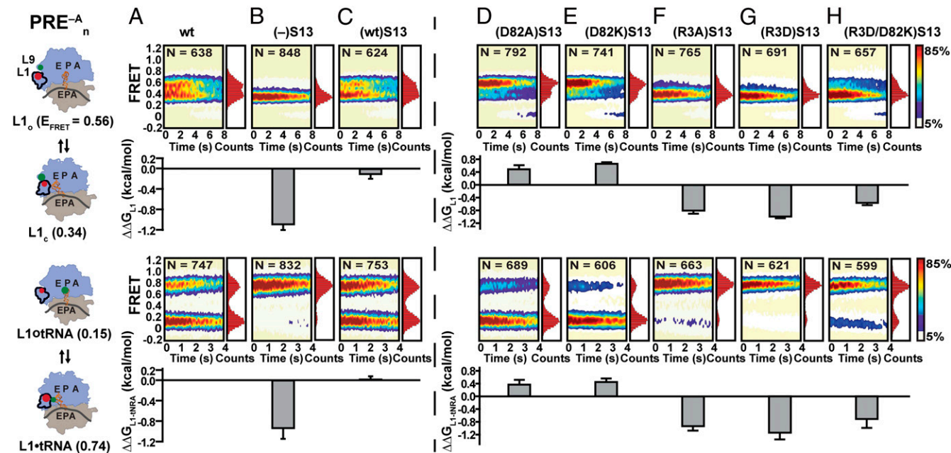
Fig. 2. (A–H) Steady-state smFRET measurements and changes in the free-energy differences of PRE -A complexes formed using (A) WT, (B) (-)S13, (C) (WT) S13, (D) (D82A)S13, (E) (D82K)S13, (F) (R3A)S13, (G) (R3D)S13, and (H) (R3D/D82K)S13 30S subunits. Cartoon representations of PRE -A complexes labeled using the smFRET L1-L9 (Upper Row) and smFRET L1-tRNA (Lower Row) labeling schemes are displayed at Left. The 30S subunit (tan); 50S subunit (light blue); L1 stalk; mRNA (gray curve); A, P, and E sites; and P-site tRNA (orange) are depicted and labeled. Surface contour plots of the time evolution of population FRET were generated by superimposing individual smFRET L1-L9 vs. time trajectories (Upper Row) and smFRET L1-tRNA vs. time trajectories (Lower Row) for each PRE -A complex. Contours are colored from white to red, denoting the lowest to highest population levels (population color bar at Far Right) and N is the number of smFRET trajectories used to construct each contour plot. The one-dimensional E_{\text{FRET}} histogram corresponding to each surface contour plot is plotted along the right-hand y axis of the surface contour plots. Bar graphs depicting the changes in the free-energy difference between L1 o and L1 c ( \Delta\Delta G_{\text{L1}} , Upper Row) and L1otRNA and L1•tRNA ( \Delta\Delta G_{\text{L1-tRNA}} , Lower Row) for each PRE -A complex relative to PRE WT -A (columns A–C) and for each PRE -A complex carrying an S13-reconstituted 30S subunit relative to PRE (WT)S13 -A (columns D–H) were generated using the \Delta\Delta G_{\text{L1}} and \Delta\Delta G_{\text{L1-tRNA}} values in Tables S2 and S3.
