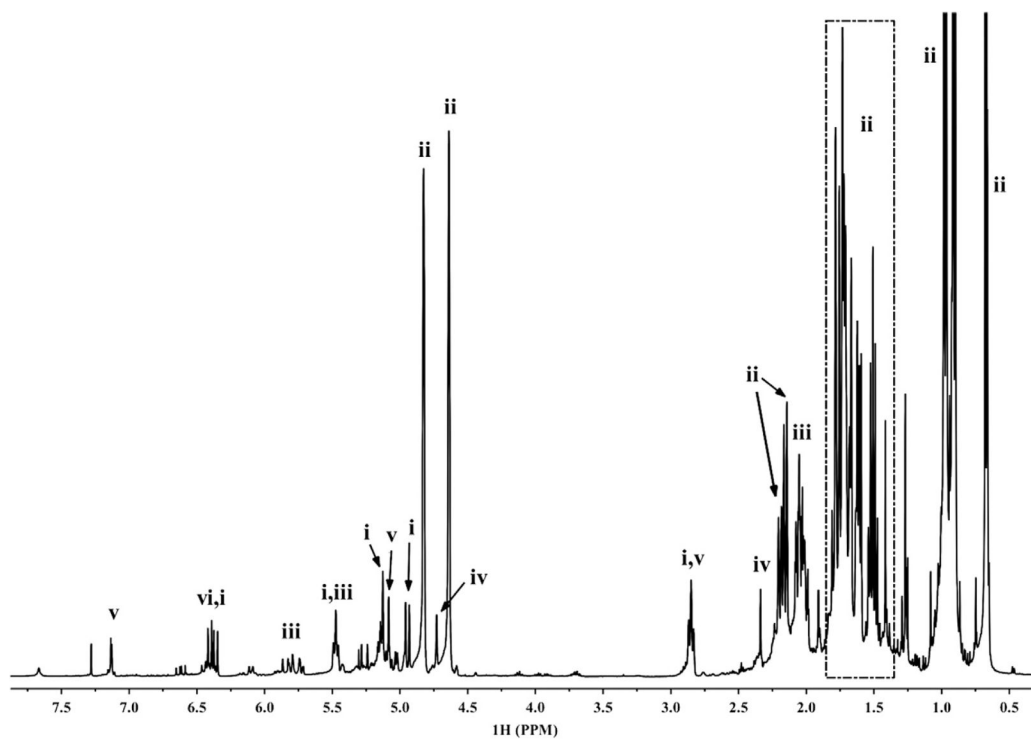
Fig. 1. 1 H NMR spectrum of pondberry essential oil and identified major components of the oil (CDCl 3 , 400 MHz). (i) ( E )-β-ocimene, (ii) sabinene, (iii) α-phellandrene, (iv) limonene, (v) p -cymene, (vi) myrcene.
