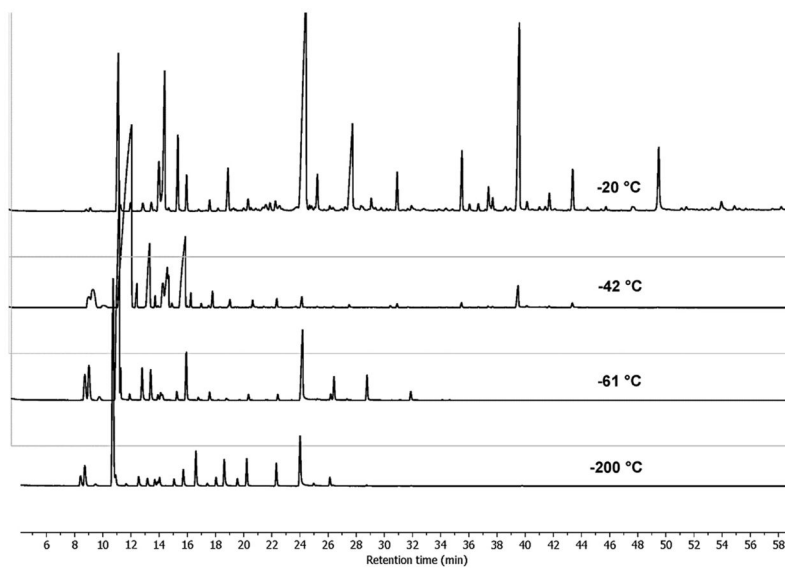
Fig. 3. GC and GC-MS chromatograms of fractions generated by fractional freezing (from top (-20 °C) to bottom (-200 °C)).
