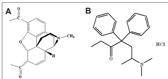
Figure 3 Chemical structure of heroin (A) and methadone hydrochloride (B).
