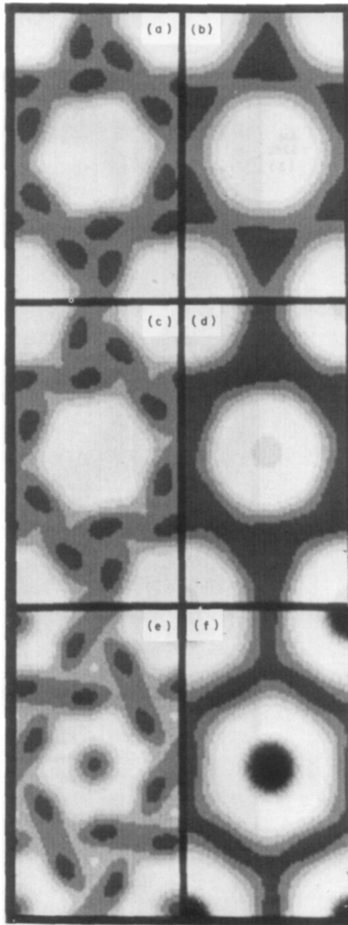
Figure 4. Fourier-averaged images from micrographs obtained at low irradiation (left column) and higher irradiation (right column) of gap junction specimens stained with: (a) and (b) methylamine tungstate; (c) and (d) phosphotungstic acid; (e) and (f) uranyl acetate.
