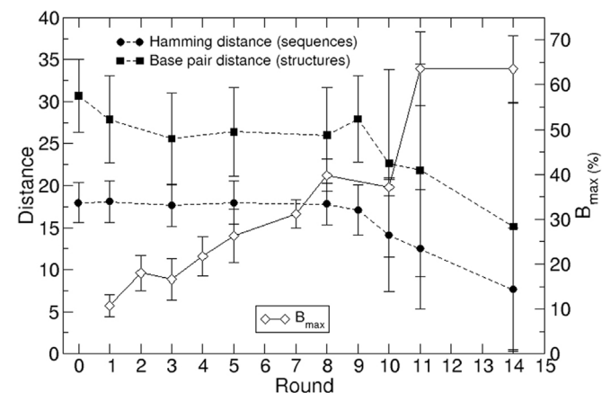
Figure 2 | Changes in relevant variables along the selection process. Average distances were computed over all possible sequence/structure pairs at each round, and error bars show the mean square deviation of each sample. In B_{\max} , error bars represent the experimental error.
