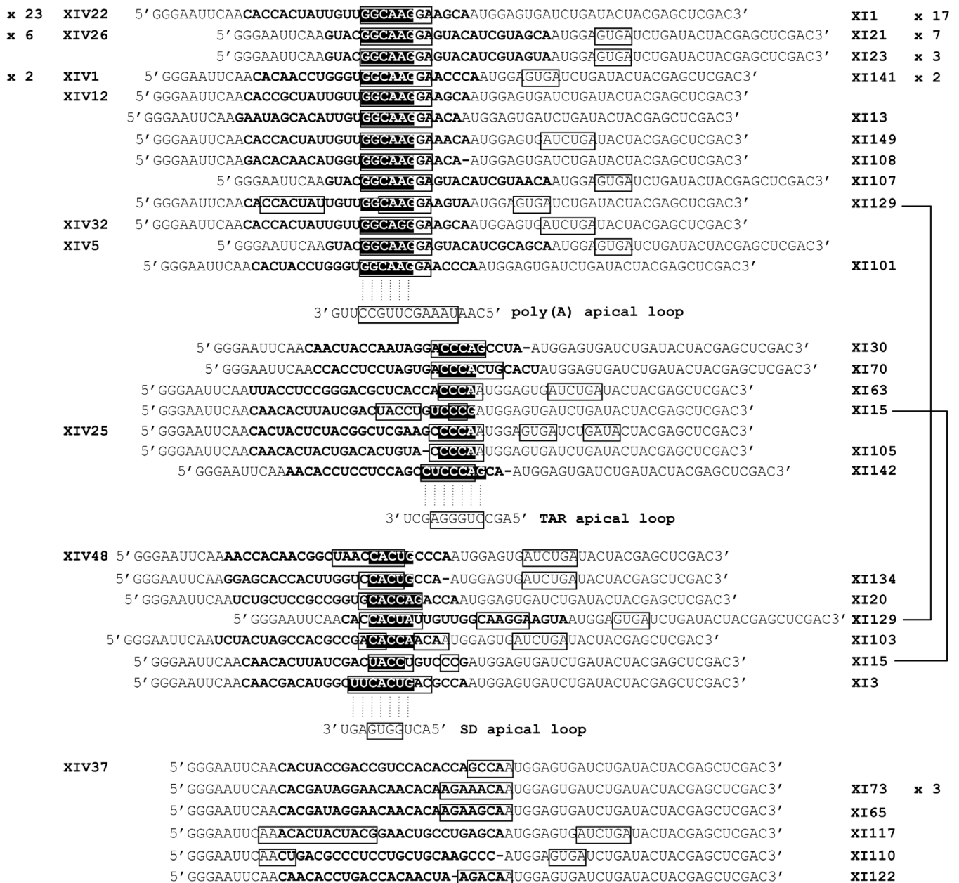
Figure 3 | Aptamer sequences of rounds XI and XIV, grouped attending to putative common targets. The variable region is shown in boldface. The single-stranded sequences predicted by RNAfold software 59 are boxed. White text represents the sequences complementary to 5'-UTR loop regions (shown below each group). xN: sequence multiplicity in each round. Among these putative interaction sites, once the energy of the folded configuration is considered (Table S2) the only robust and energetically favoured interaction is that with the poly(A) apical loop.
