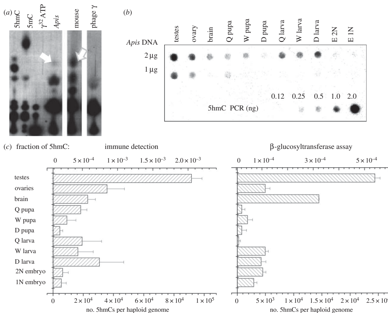
Figure 1. (a) TLC identification of 5hmC in A. mellifera . Single radiolabelled nucleotides derived from a variety of samples were separated by TLC on PEI cellulose. Samples obtained from single dNTPs were used as standards. Three genomic DNA preparations were digested to single nucleotides and immunoprecipitated with anti-5hmC antibodies. Purified nucleotides were radiolabelled and resolved by TLC. A spot representing 5hmC is present in drone testes DNA, whereas a much stronger spot can be seen for mouse brain known to be enriched in 5hmC (white arrows). No 5hmC spot can be found in \lambda phage (Dam - Dcm - ). All lanes are from the same TLC plate. (b) An image of a DNA dot-blot hybridized with an anti-5hmC antibody. For each sample, 1 and 2 \mu g of DNA were spotted on the membrane. A PCR product with dCTP substituted for d5hmCTP was used as control. (c) 5hmC quantification in various honeybee DNA samples. The data points were obtained using two methods; a densitometry scan of the dot-blot shown in (b), and a \beta -glucosyltransferase assay (see Material and methods). The resulting values were plotted as either fractions of total cytosines (top) or as a number of 5hmCs in a haploid genome (bottom). The overall correlation between two methods is 0.712. Q, W, D and E refer to queen, worker, drone and embryos, respectively.
