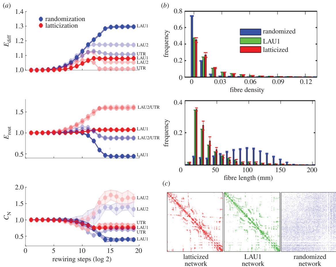
Figure 2. (a) Latticization and randomization of empirical brain networks. (b) Fibre length and fibre density distributions of randomized networks (blue), LAU1 network (green) and latticized networks (red). Randomized and latticized network distributions are averages over 40 repetitions of the randomization and latticization process applied to the LAU1 empirical network. (c) Adjacency matrices of latticized LAU1 network (red), LAU1 network (green) and randomized LAU1 network (blue).
