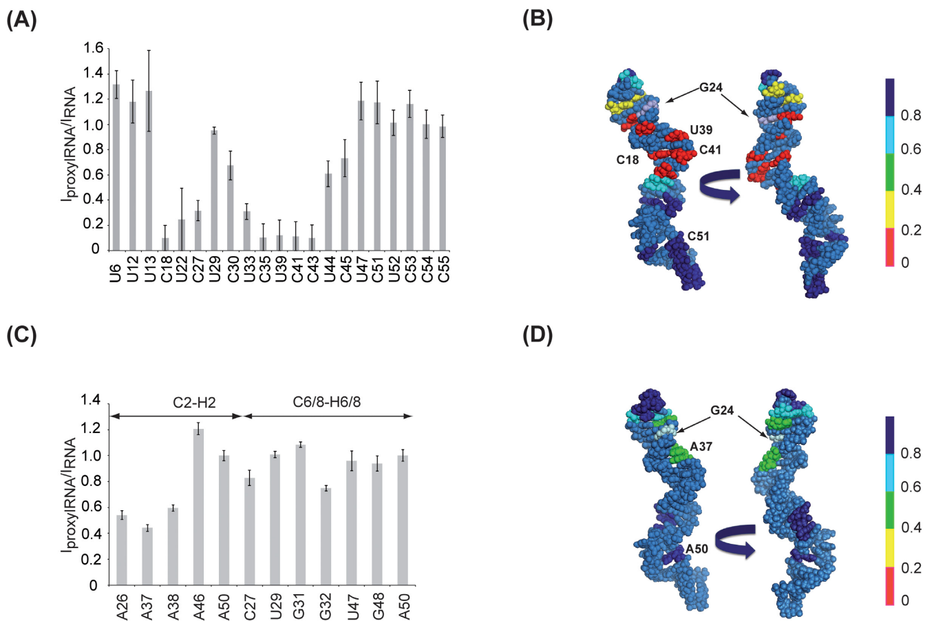
Figure 6. Effect of site-specific spin-labeled RNA analyzed by NMR. (A) Bar graph of intensity ratio between the spin-labeled RNA ( I_{\text{proxyl}}/I_{\text{RNA}} ) and the free form RNA ( I_{\text{RNA}} ), normalized to C54, extracted from MLEV experiments, versus the primary sequence of the RNA. The quantification of residues C18, U22, C35, U39, C41 and C43 was not feasible due to the disappearance of the corresponding resonances. The corresponding ratios were estimated by measuring values at the same frequencies as the resonances observable in the wild-type RNA. (B) Sphere representation of the RNA structure colored according to the intensity ratios extracted from MLEV experiments. The spin-labeled G24 residue is highlighted in light blue. (C) Bar graph of intensity ratio between the (G1-A23)-(G24 6 TG proxyl -C55) RNA and the free form RNA, normalized to A50, extracted from HSQC experiment, versus the primary sequence of the RNA. (D) Sphere representation of the RNA structure colored according to the intensity ratios extracted from HSQC experiments. The spin-labeled G24 residue is highlighted in light blue.
