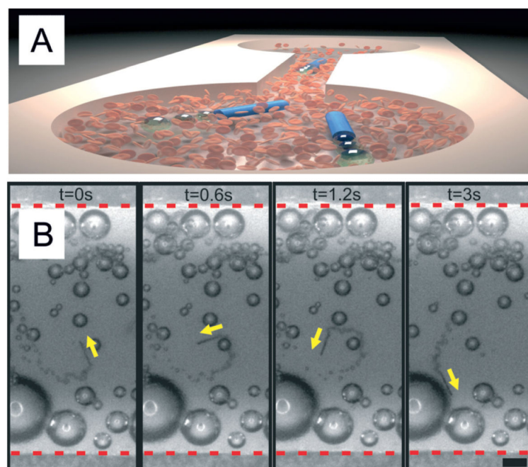
Fig. 4. Microjets moving together with diluted blood in microfluidic chips. A) Sketch of the motion of microjets moving from one side to the other of the microchip. B) Optical microscope images of a microjet engine moving against the flow in a microfluidic channel with blood 10× diluted at 37 °C. Scale bar: 50 μm.
