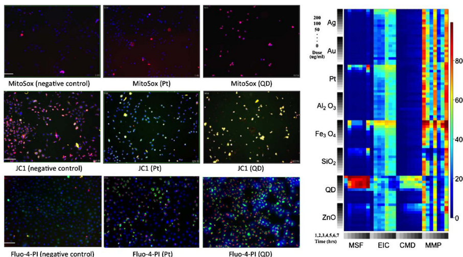
Fig. 1. Fluorescence images and heat map of raw data. On the left are fluorescence images of RAW cells treated with various nanomaterials (quantum dot, platinum and a negative control) and dyed with compatible dye combinations including MitoSox, JC1, PI and Fluo-4. The subsequent fluorescence read-out, measured at varying wavelengths, provides a measure of the number of cells positive for the response. On the right is a heat map of the raw data for each particle and outcome. Colder colors indicate a smaller percentage of cells positive for the response and warmer colors indicate a larger percentage of cells positive for the response.
