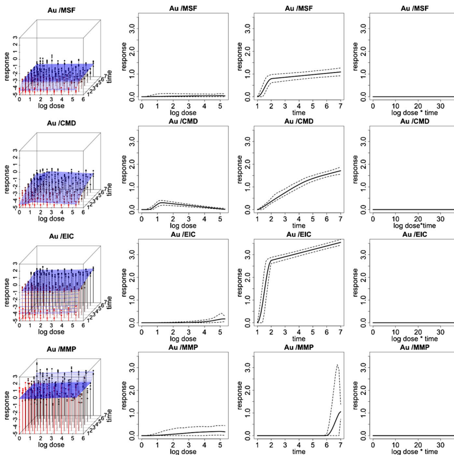
Fig. 4. Fitted response curves for the gold (Au) ENM. Fitted response surfaces (column 1), dose-response function, f_{ij}(d) (column 2), duration-response function, g_{ij}(t) (column 3), dose/duration interaction function, h_{ij}(dt) (column 4) and associated 95% posterior intervals. In (column 1), the color red represents response values corresponding to lower time points and the color black represents response values corresponding to higher time points.
