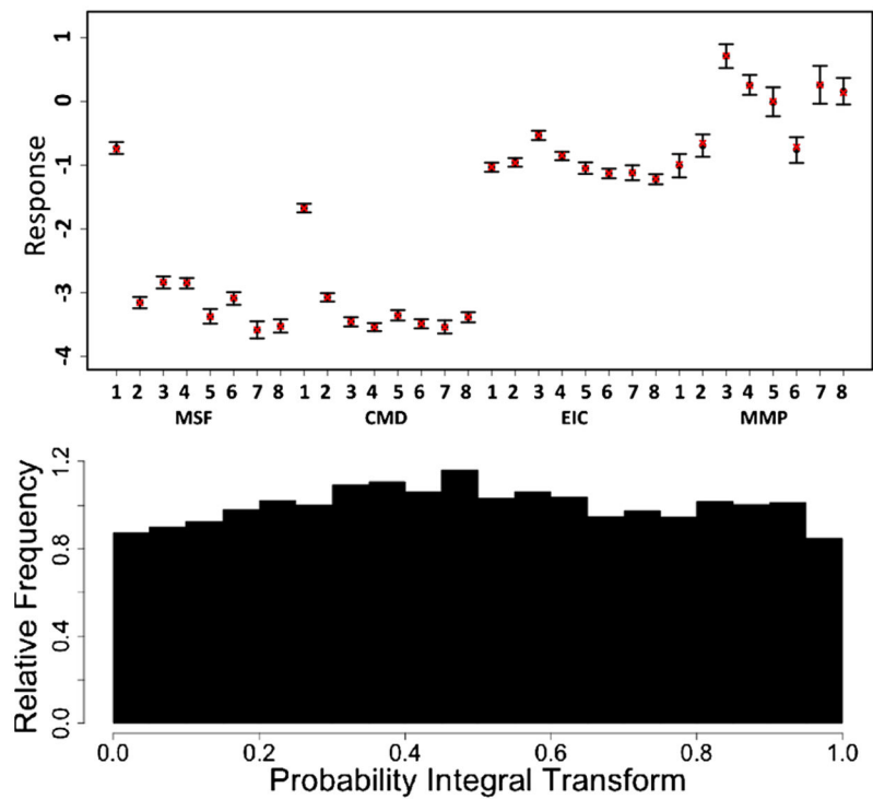
Fig. 5. Graphical model diagnostics. (Bottom) Probability Integral Transform assessing empirical calibration of the posterior predictive distribution. (Top) Mean and 95% posterior intervals of the posterior predictive mean response across all doses and times of exposure, for all outcomes and particles 1 through 8 (QD, ZnO, Fe 3 O 4 , Pt, Ag, SiO 2 , Al 2 O 3 , Au). Also included are the empirical mean responses across all doses and times of exposure (red).
