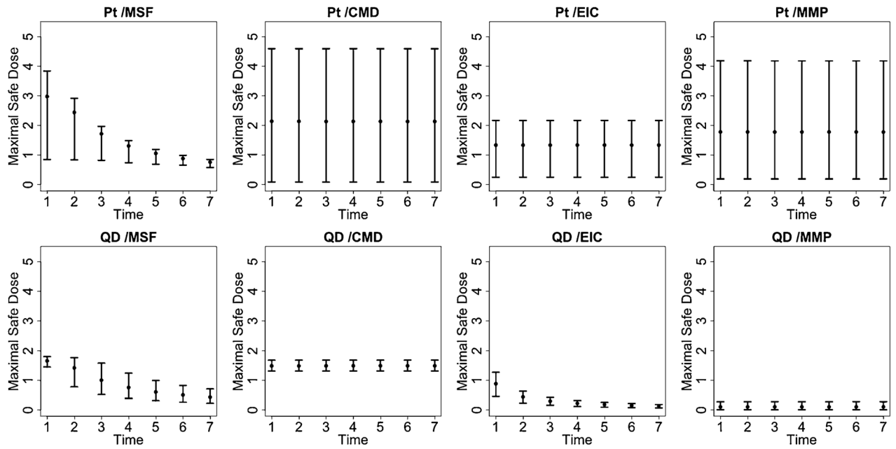
Fig. 7. Maximal Safe Dose for the quantum dot (QD) and platinum (Pt) nanomaterials. Posterior summary estimates of the maximal safe dose, conditional on exposure time, including the posterior mean and associated 95% posterior intervals. In the case of no interaction, the maximal safe dose is the same across all times.
