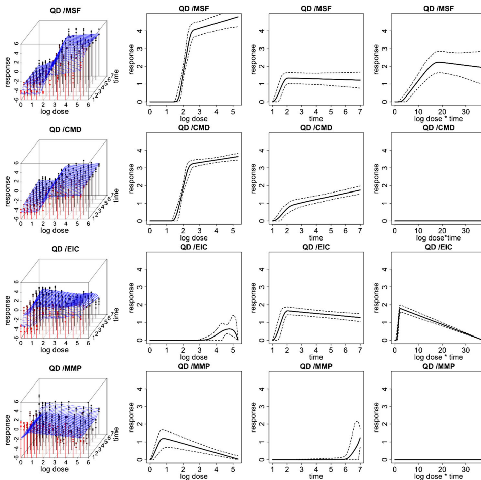
Fig. 3. Fitted response curves for the quantum dot (QD) ENM. (left) Fitted response surfaces (column 1), dose-response function, f_{ij}(d) (column 2), duration-response function, g_{ij}(t) (column 3), dose/duration interaction function, h_{ij}(dt) (column 4) and associated 95% posterior intervals. In (column 1), the color red represents response values corresponding to lower time points and the color black represents response values corresponding to higher time points.
