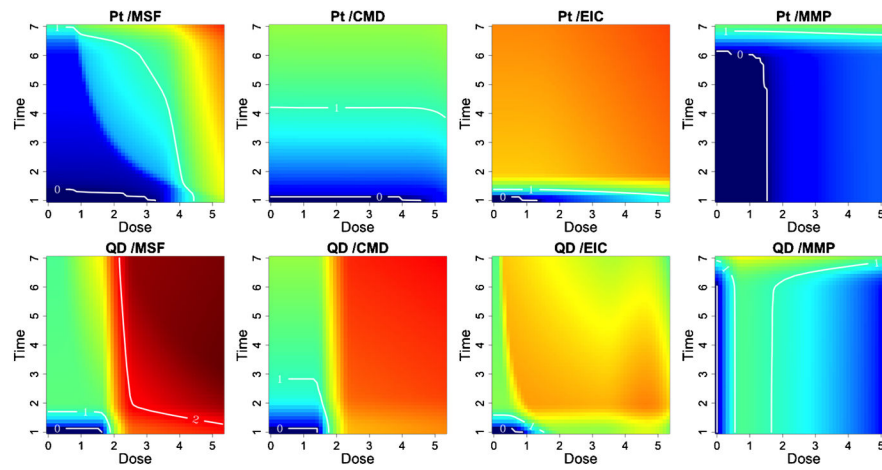
Fig. 6. Safe exposure regions for the quantum dot (QD) and platinum (Pt) nanomaterials. For each particle and outcome we can define dose and time exposure regions which do not induce cytotoxicity. Red colored regions indicate greater cytotoxicity to the cells, whereas blue colored regions indicate reduced risk. Contour lines quantitate the median estimated response, relative to the background, where zero response areas can be interpreted as safe exposure regions.
